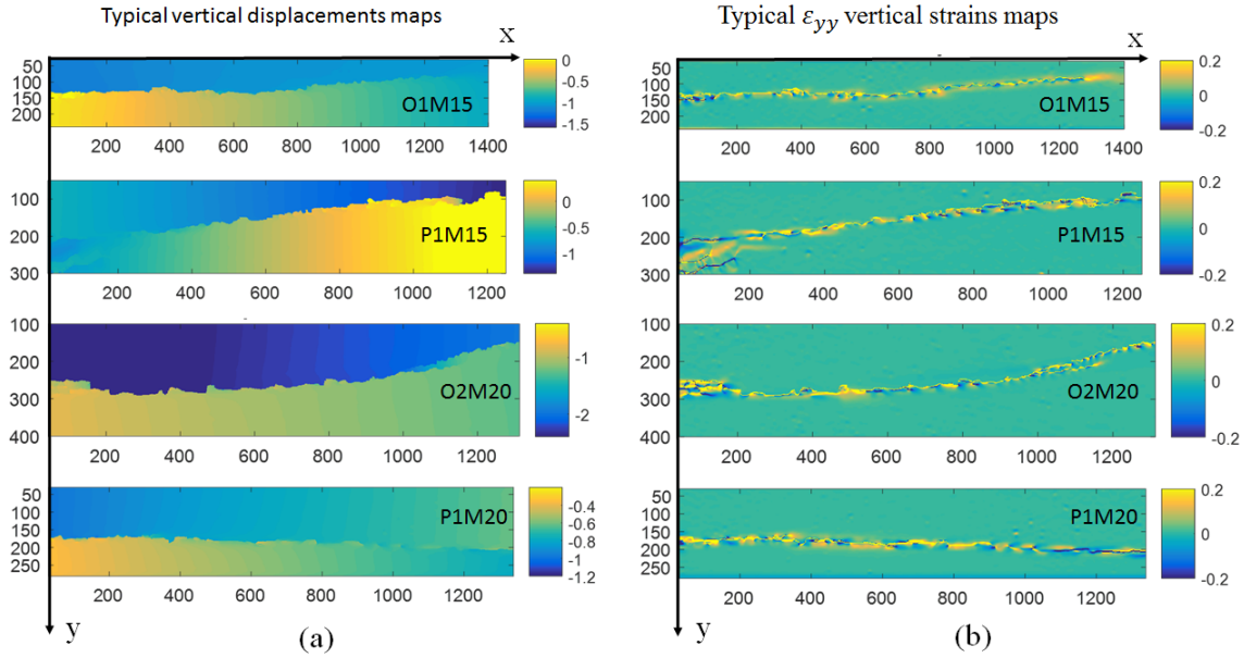
Figure 16: Typical maps for MMCG specimens at the end of the tests : a) displacement maps; b) strain maps.
