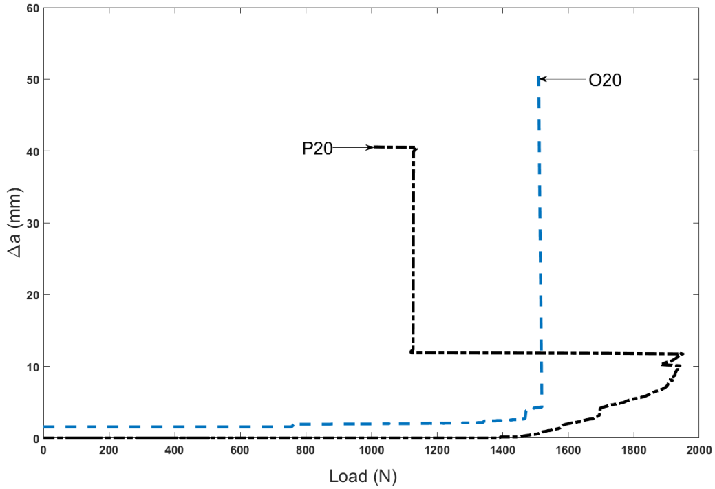
Figure 21: Example of crack length as a function of the load for two CTS specimens (Thickness 20 mm).
