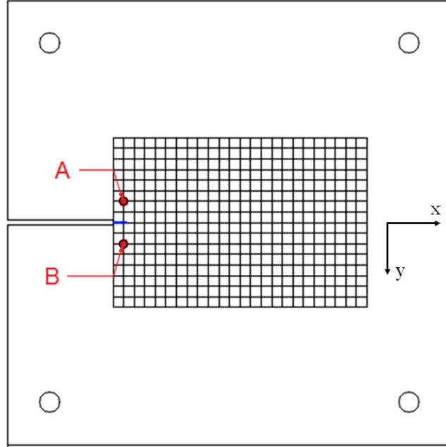
Figure 11: Points A and B used for determination of the crack opening U .
