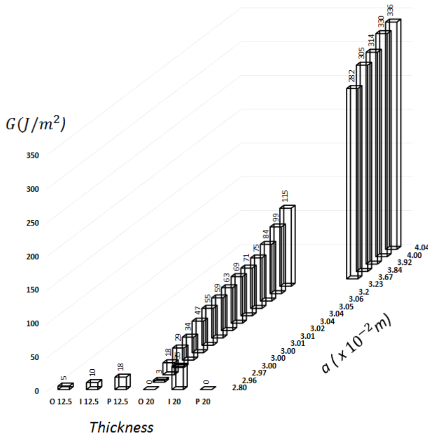
Figure 23: Critical energy release rate of Okume (O), Iroko (I) and Padouk (P) (thickness 12.5 mm and 20 mm).
