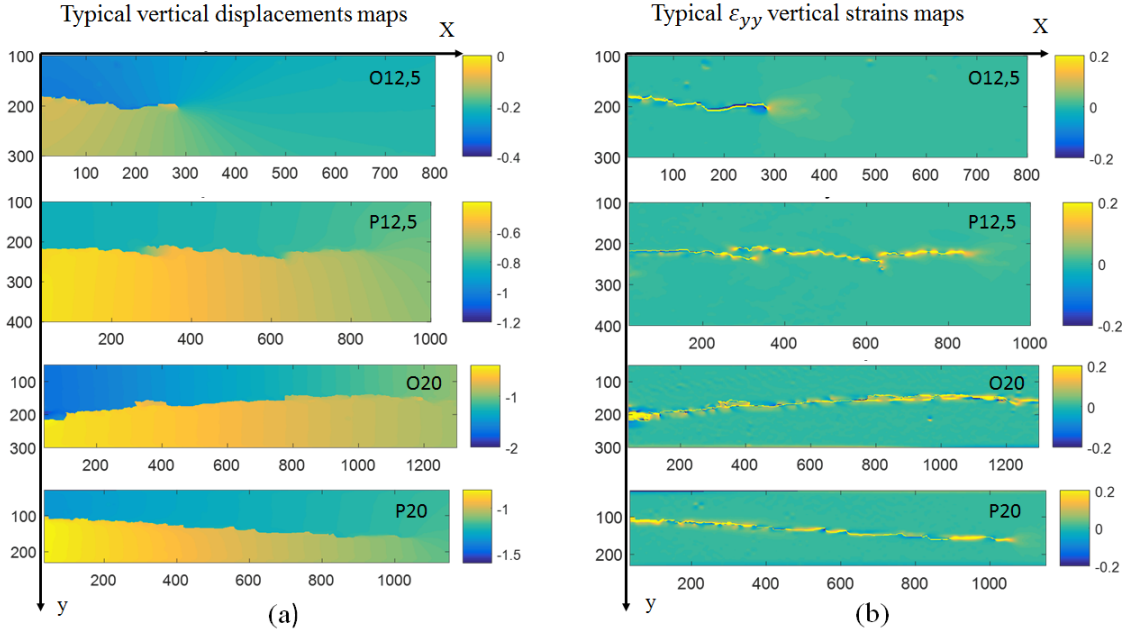
Figure 15: Typical maps for CTS specimens at the end of the tests : a) displacement maps; b) strain maps.
