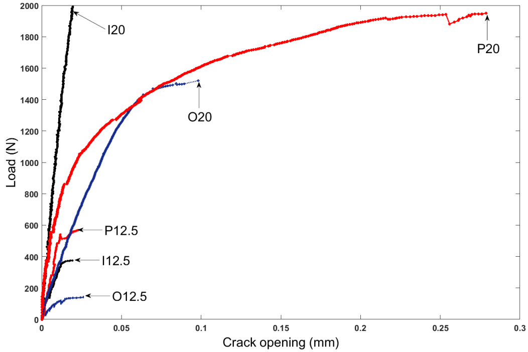
Figure 17: Load - crack opening curves for the CTS specimens.
