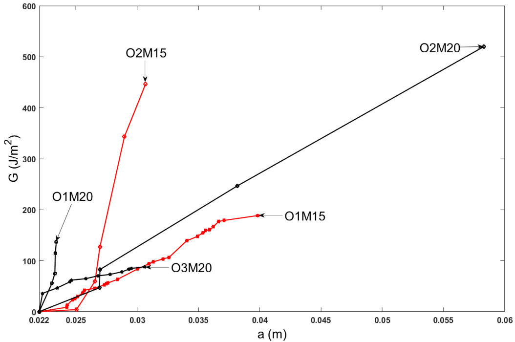
Figure 24: Critical energy release rate G_c as a function of the crack length for Okume (O).
