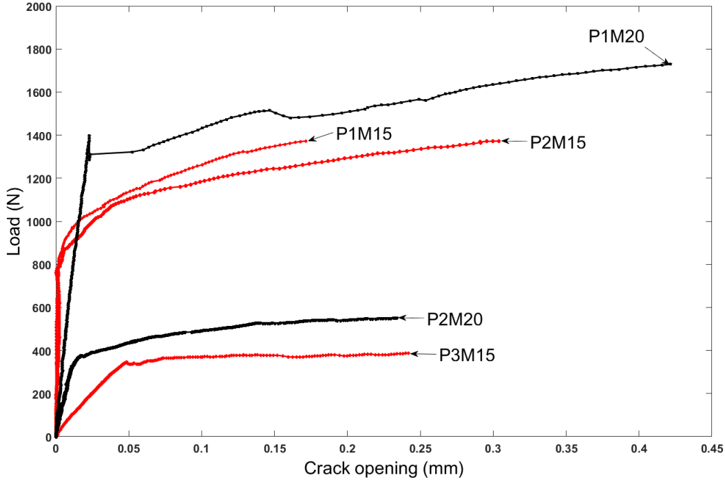
Figure 20: Load - crack opening curves for the MMCG Padouk specimens and two thicknesses (15 mm and 20 mm).
