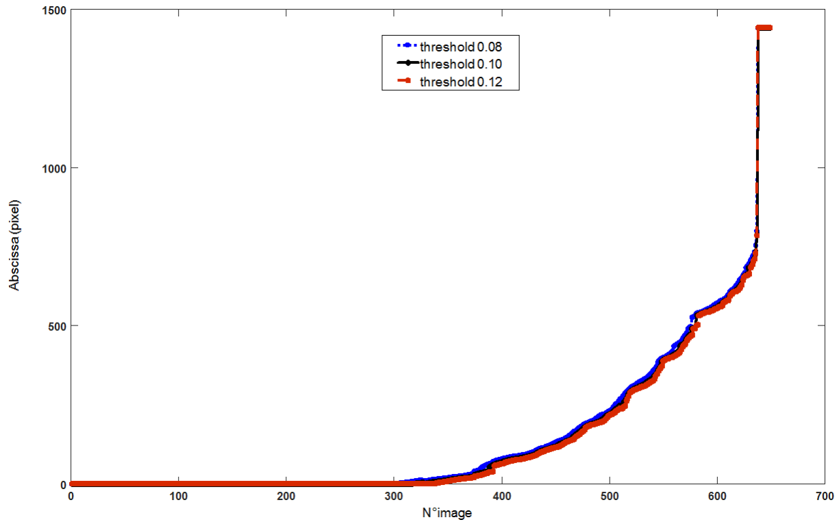
Figure 12: Abscissa of the crack tip obtained for three different threshold values of \varepsilon_{yy} .
