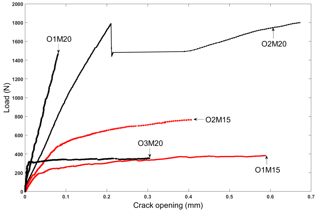
Figure 18: Load - crack opening curves for the MMCG Okume specimens and two thicknesses (15 mm and 20 mm).
