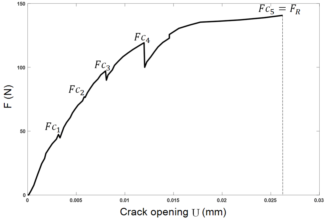
Figure 10: Force versus the crack opening U .
