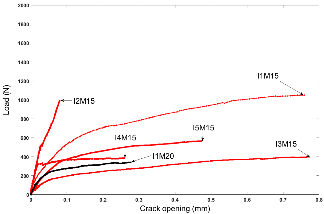
Figure 19: Load - crack opening curves for the MMCG Iroko specimens and two thicknesses (15 mm and 20 mm).
