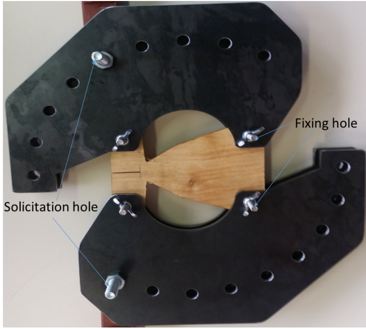
Figure 8: MMCG specimen and Arcan fixture.
