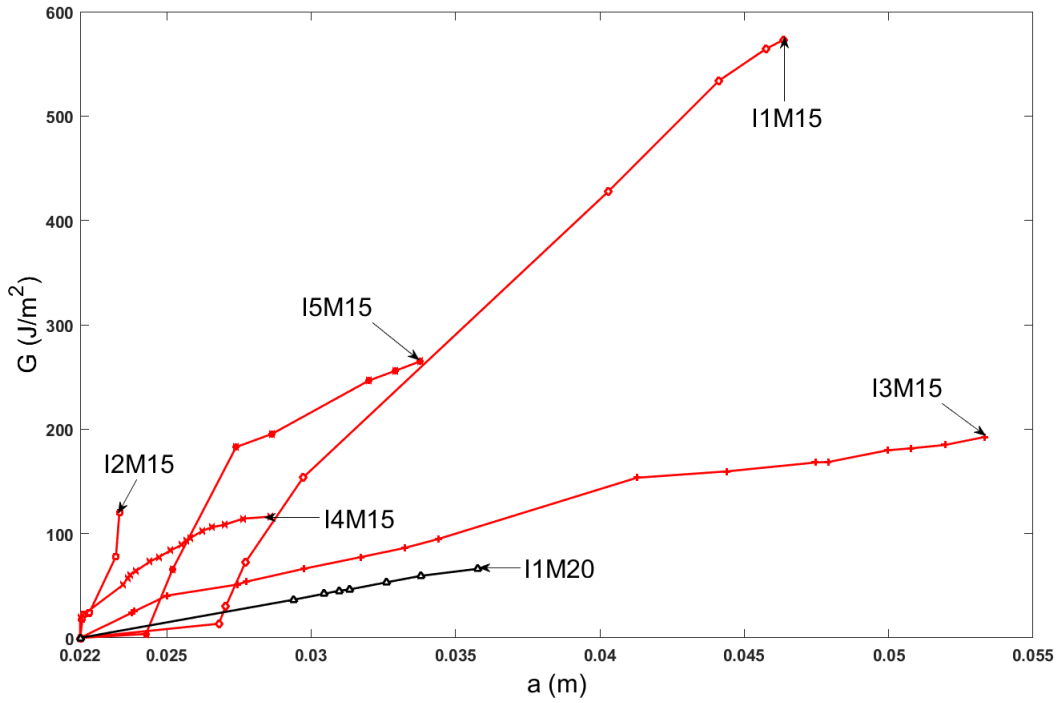
Figure 25: Critical energy release rate G_c as a function of the crack length for Iroko (I).
