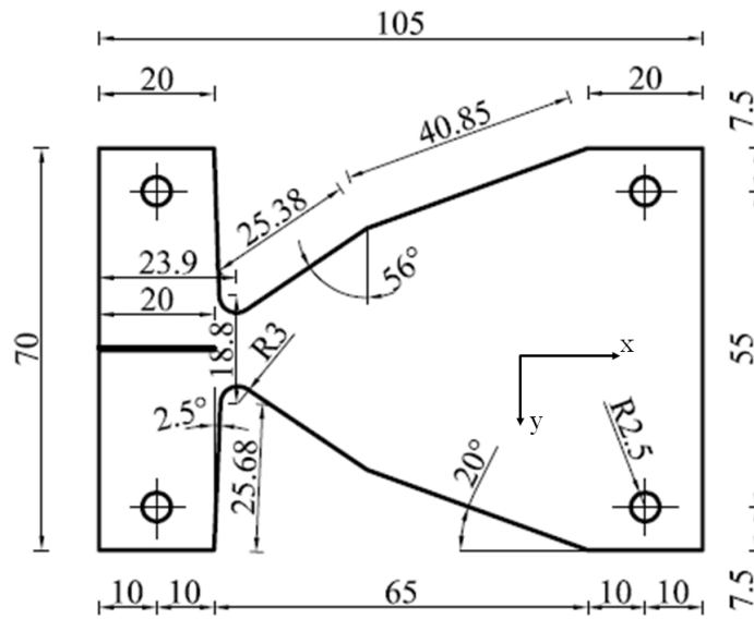
Figure 4: Dimensions of the modified MMCG specimen (in mm).
