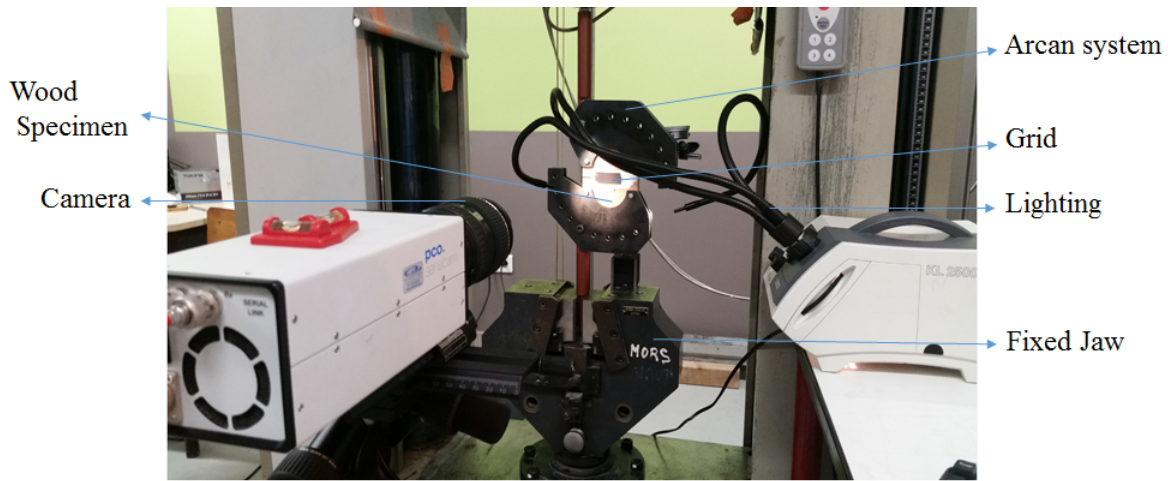
Figure 14: Experimental setup.
