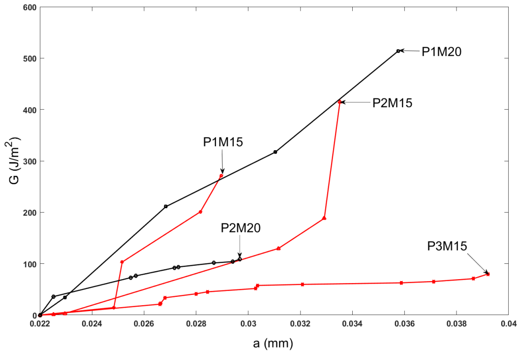
Figure 26: Critical energy release rate G_c as a function of the crack length for Padouk (P).
