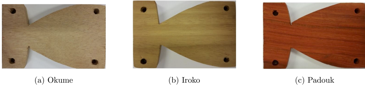
Figure 5: Typical MMCG specimens for three wood species: Okume, Iroko and Padouk.
