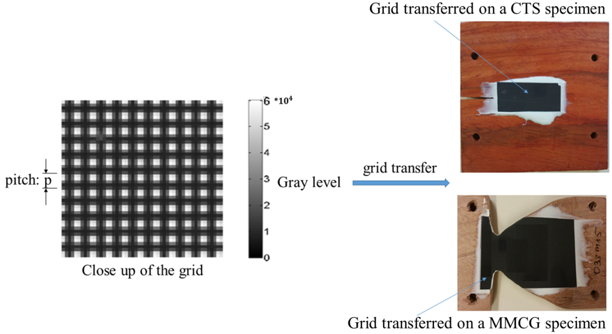
Figure 9: Typical examples of grid transferred on CTS and MMCG specimens.
