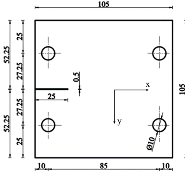
Figure 2: Dimensions of the CTS specimen (in mm).
