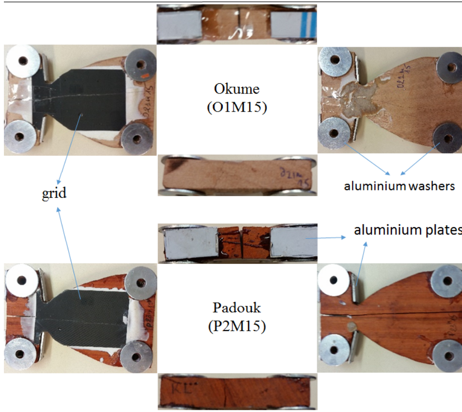
Figure 6: Typical MMCG specimens equipped with grids.
