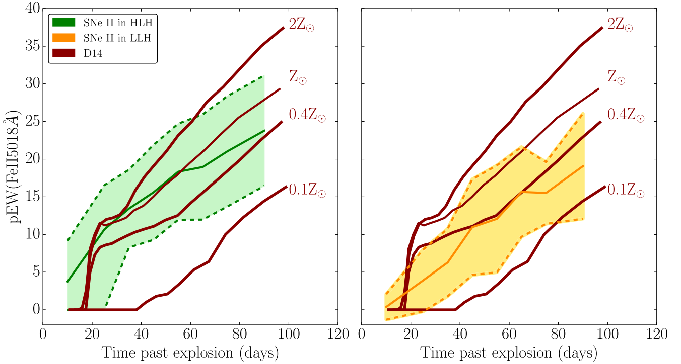
Figure 6. Temporal evolution of pEW(\text{Fe II } 5018 \text{ \AA}) from explosion to +90 d, in both the data and models at four different metallicities. The observational data are binned in time. Left: Comparison between the SNe II in high-luminosity hosts. The green solid line represent the mean of the pEW within each time bin, while the dashed green lines indicate the standard deviation. Right: The comparison with SNe II in low-luminosity hosts, with the mean of the pEW orange solid line and the standard deviation in dashed orange lines. In both panels, the brown solid lines represent the D14 models as labelled.
