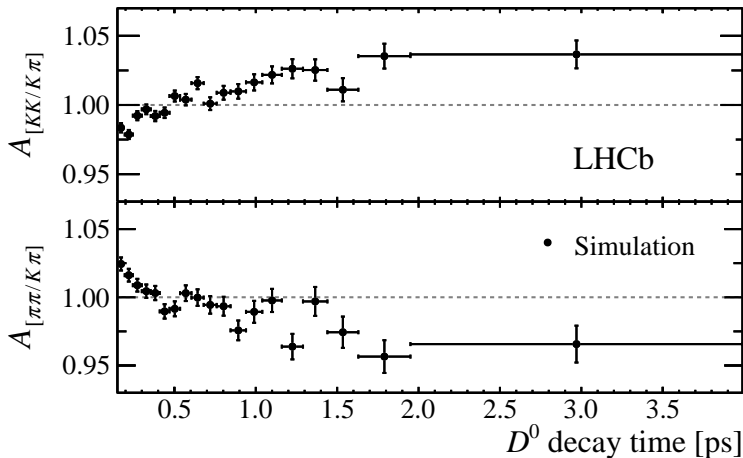
Figure 2: Ratio of decay-time acceptances from simulation for (top) D^0 \rightarrow K^+K^- over D^0 \rightarrow K^-\pi^+ decays and (bottom) D^0 \rightarrow \pi^+\pi^- over D^0 \rightarrow K^-\pi^+ decays.
