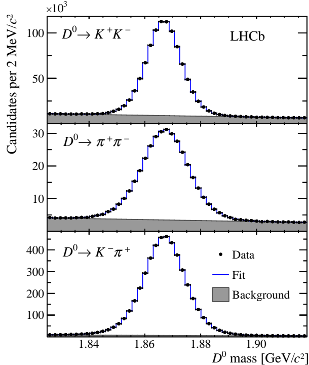
Figure 1: Distribution of D^0 mass for candidates passing the selection with fit projections overlaid: (top) D^0 \rightarrow K^+K^- decays, (center) D^0 \rightarrow \pi^+\pi^- decays, and (bottom) D^0 \rightarrow K^-\pi^+ decays.
