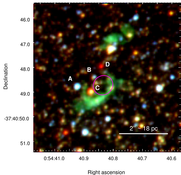
Figure 4. Top panel: HST /ACS-WFC RGB colour image of S 10. Red represents the F814W band, green is the F606W band, and blue is the F475W band. Overlaid are the ATCA 5.5 GHz contours in white and, in magenta, the 95 per cent confidence Chandra error circles (Section 2.4) for the peak-emission location of each knot. There is nebular emission (likely H\alpha plus [N II], which are covered by the F606W bandpass) coincident with X-ray knot 2 and the peak radio emission. The star-forming region and photoionized nebula H 10 (Blair & Long 1997) are to the south-west. Bottom panel: Zoomed-in image of the inner part of the S 10 complex around the extended X-ray knot 2, more clearly showing the two separate nebulae (in green). The magenta circle represents the 95 per cent confidence Chandra central position of the brightest knot (Section 3.3.2). Letters indicate potential optical counterparts for the accreting compact object, origin of the jet. The distinct morphology of the line-emitting nebula around the peak X-ray and radio emission could be a result of anisotropic ejecta from a progenitor SN or it could be gas shock-ionized by the jet and the counterjet.
