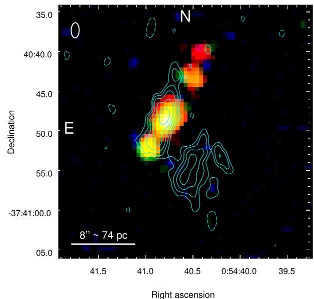
Figure 2. Top panel: Stacked Chandra ACIS-I image of NGC 300 S 10. Red represents 0.3–1.0, green 1–2, and blue 2–7 keV. The image has been adaptively smoothed with a Gaussian kernel of \sigma = 1 pixel and has a pixel size of 0''.492 . Cyan contours show the ATCA 5.5 GHz map; contour levels are 2\sigma \times \sqrt{2}'' , where \sigma = 2.72 \mu\text{Jy beam}^{-1} . The beam size is 2''.91 \times 1''.47 . Similarly to the H\alpha emission (Fig. 1), the radio emission consists of a component associated and aligned with the X-ray knots in the S 10 region, plus a component associated with the H 10 H II region (Blair & Long 1997) and another component corresponding to the S 9 SNR (Blair & Long 1997). Bottom panel: Same as the top panel, but the contours are now from the ATCA 9 GHz map; contour levels are 2\sigma \times \sqrt{2}'' , where \sigma = 2.78 \mu\text{Jy beam}^{-1} . The beam size is 1''.91 \times 1''.01 . The radio emission at S 10 is spatially resolved both along the direction of the jet, and in the transverse direction, both at 5.5 and at 9 GHz.
