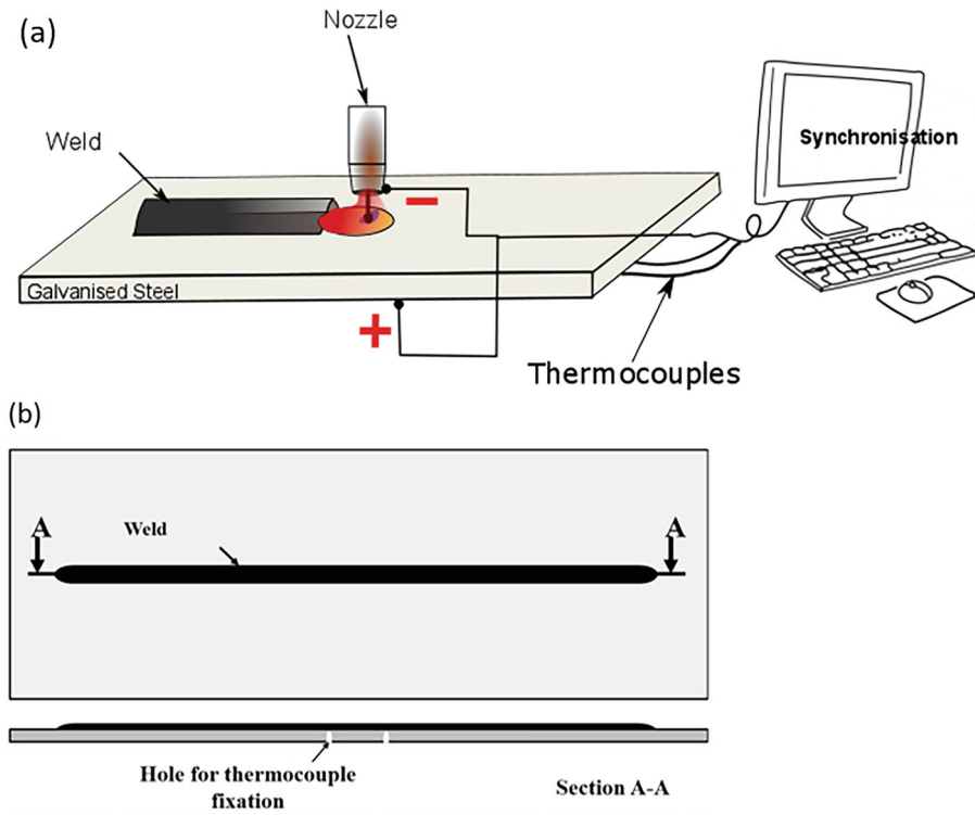
Figure 1. (a) Experimental set-up scheme, (b) weld and thermocouples location.
