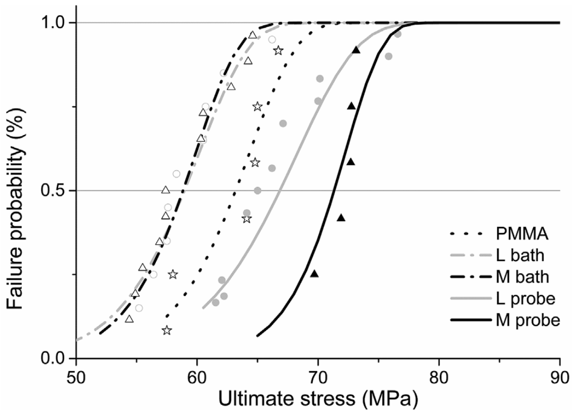
Fig.12. Weibull prediction
