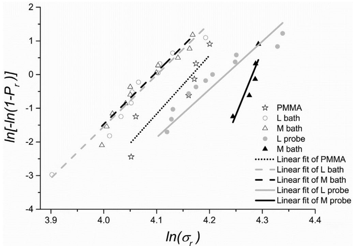
Fig.11. Accumulated Weibull probability plots for the failure stress, in MPa
