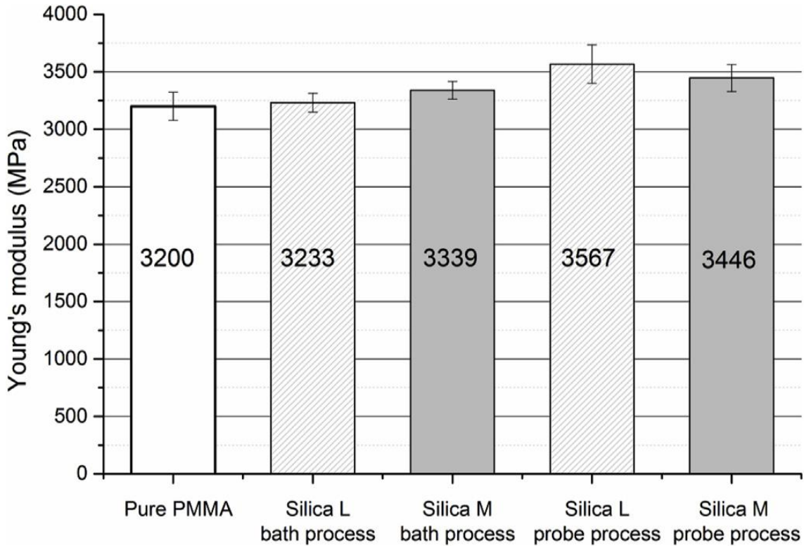
Fig9.Process impact and size effect on Young's modulus
