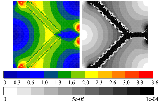
Fig. 11. The norm of the couple-stress \mathbf{m} (in MPa) and the norm of the curvature tensor \|\boldsymbol{\kappa}\| (right) at time \bar{t} = 50 (left). The scale for normalized \|\boldsymbol{\kappa}\| has been set so that the maximum value is 10^{-4} corresponding to the cutoff in the numerical regularization. There is some irregularity in the cutoff region which may be in part due to the interpolation from the integration points of the finite elements to the nodes but also to actual noise in the solution.
