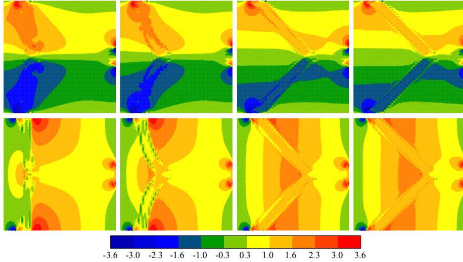
Fig. 10. The non-zero contributions to the couple-stress \mathbf{m} \in [-3.6, 3.6] MPa at time \bar{t} = 0.1, 1, 10 and 50 (left to right). The top row shows the x -component ( m_{zx} ) and the bottom row shows the y -component ( m_{zy} ).
