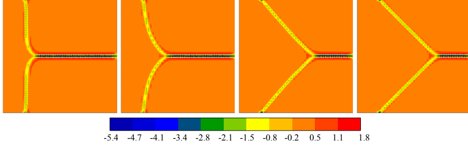
Fig. 7. Microstress \pi_\phi \in [-5.4, 1.8] MPa at time \bar{t} = 0.1, 1, 10 and 50 (left to right). Note that as the solution stabilizes, the dissipative part \pi_\phi^{neq} goes to zero and only the energetic contribution remains.
