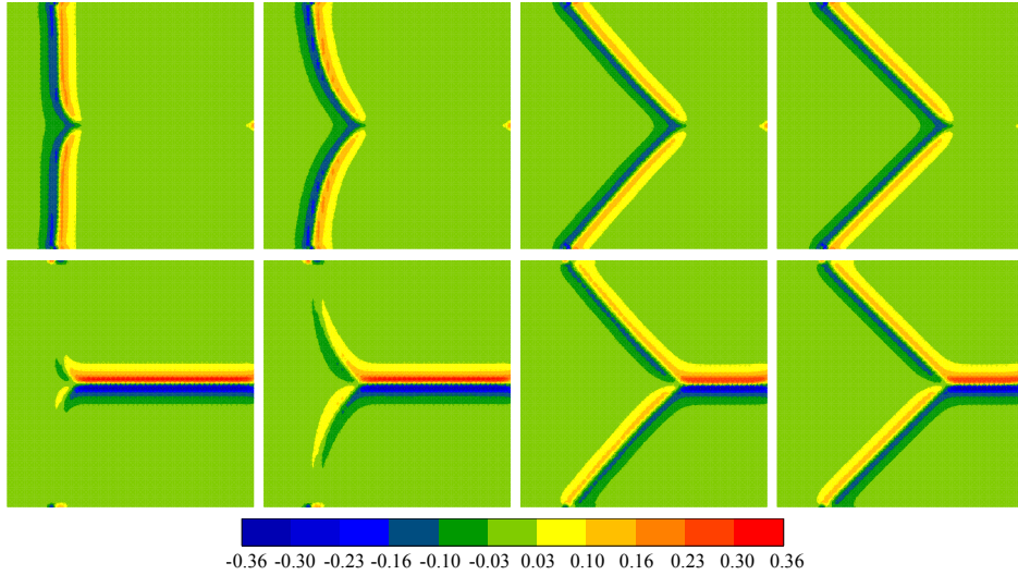
Fig. 8. Microstress \underline{\xi}_\phi \in [-0.36, 0.36] MPa at time \bar{t} = 0.1, 1, 10 and 50 (left to right). The top row shows the x -component and the bottom row shows the y -component.
