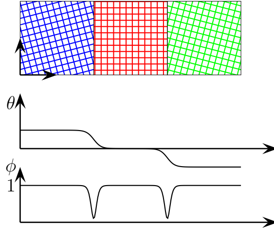
Fig. 1. Schematic representation of the profiles of the orientation \theta and order parameter \phi phase fields in the KWC model for a single-phase solid polycrystal.
