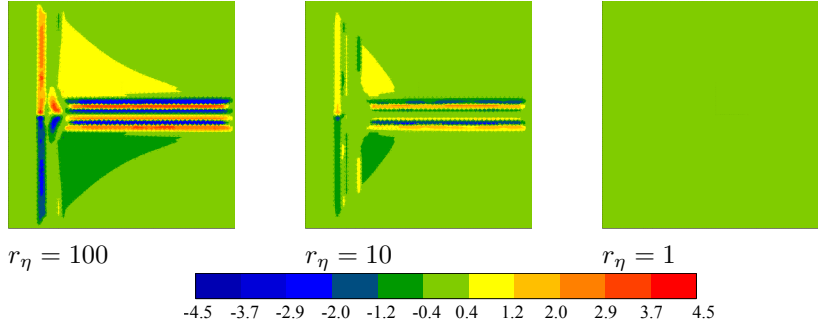
Fig. 9. Skew-symmetric stress contribution \check{\sigma} (in MPa) at \bar{t} = 0.1 for three different values of r_\eta = \hat{\eta}_*/\eta_\phi . From left to right, top to bottom: r_\eta = 100, 10 and 1 .
