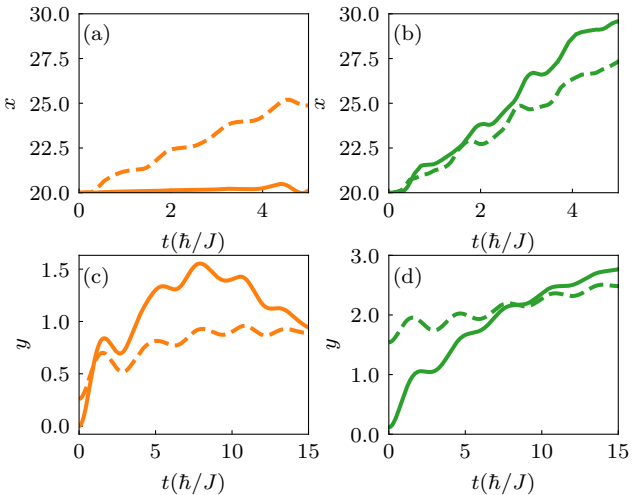
FIG. 6. Time evolution of the center-of-mass in x -direction on the edge line and y -direction for the single-particle (a,c) and FCI (b,d) phase. Solid (dashed) lines correspond to the cases with \mu = -100J ( \mu = -2J ).
