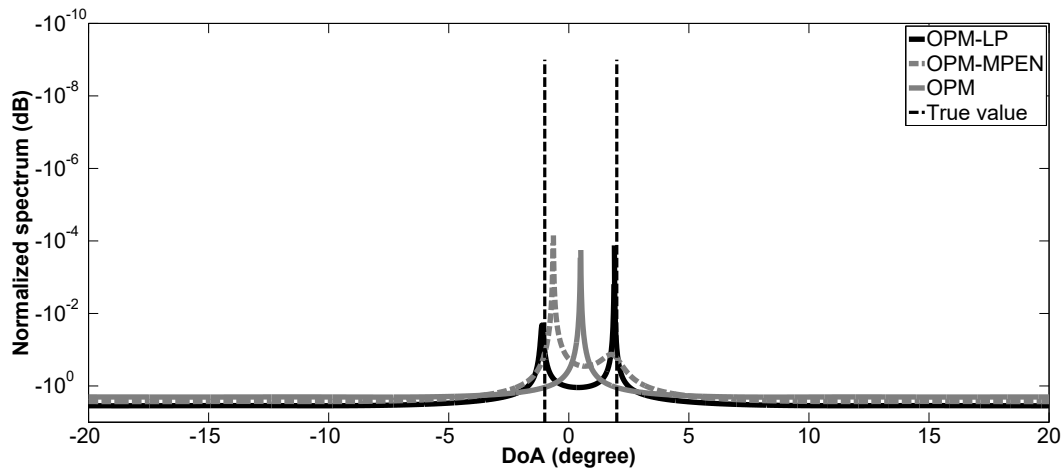
Figure 4: Case b , pseudo-spectrums of the OPM-LP, conventional OPM and OPM-MPEN for DoA estimation, the two DoAs are \theta_1 = -1^\circ and \theta_2 = 2^\circ .
