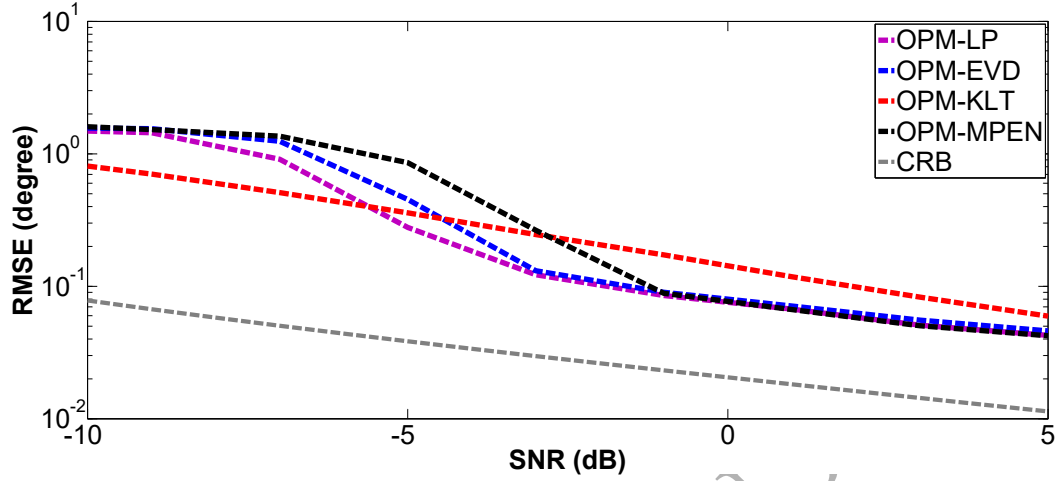
Figure 5: Case b , RMSE of DoA estimation versus SNR
