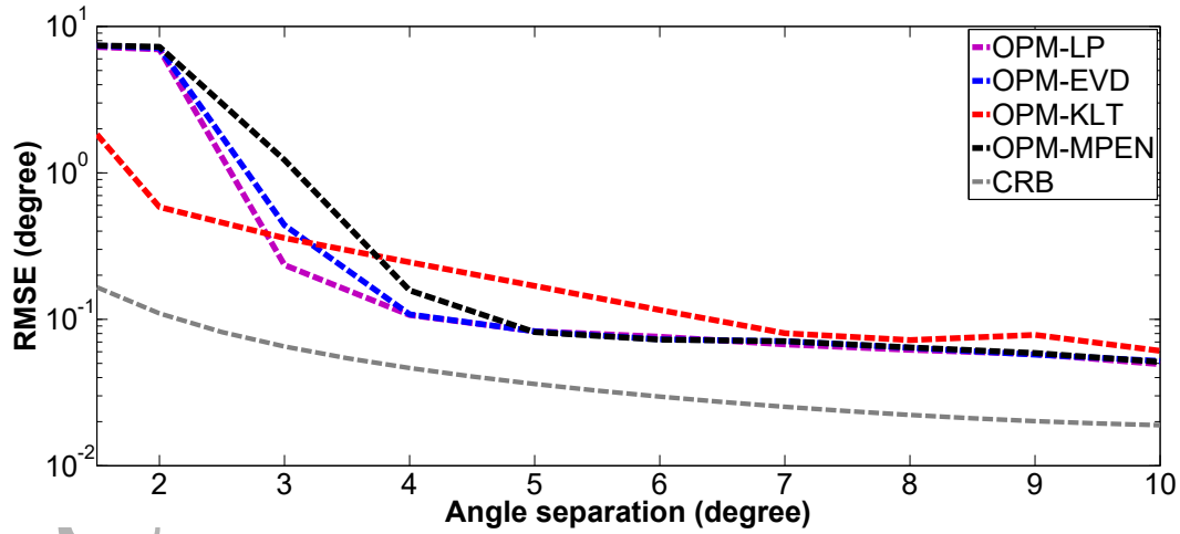
Figure 6: RMSE of DoA estimation in terms of angle separation
