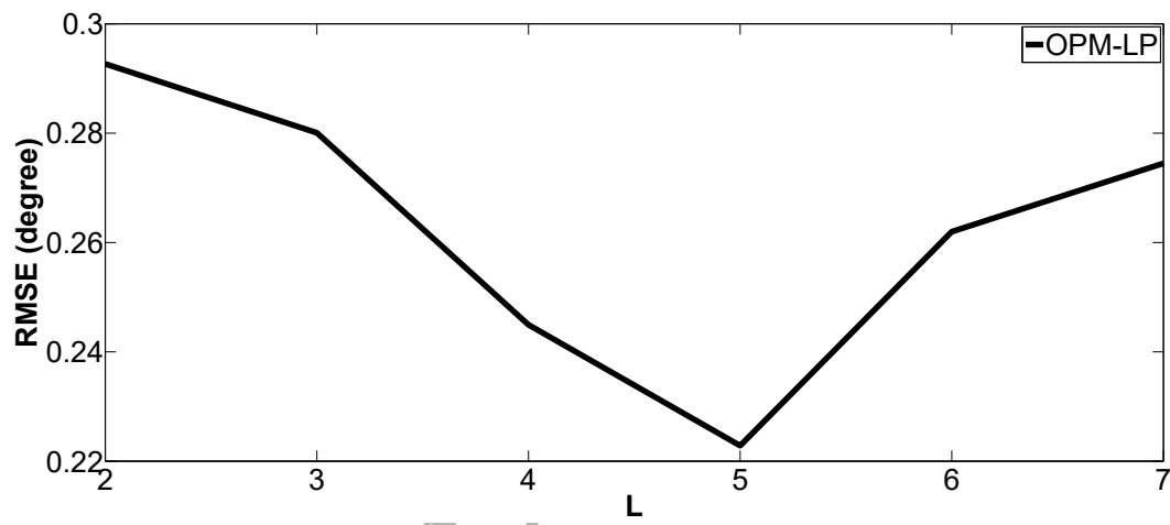
Figure 7: RMSE of DoA estimation as a function of L
