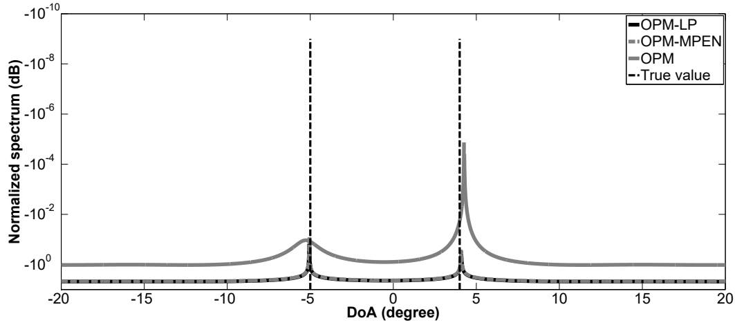
Figure 3: Case a , pseudo-spectrums of the OPM-LP, conventional OPM and OPM-MPEN for DoA estimation, the two DoAs are \theta_1 = -5^\circ and \theta_2 = 4^\circ .
