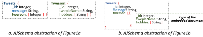
Fig. 3: AJSchemas for examples presented in Figure 1
