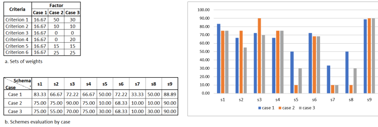
Fig. 8: Schema evaluation
