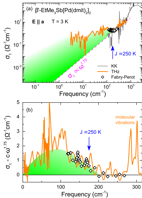
FIG. 3: (a) Low-temperature conductivity spectra of \beta' -EtMe 3 Sb[Pd(dmit) 2 ] 2 plotted in a broad range. The black line corresponds to Kramers-Kronig results from optical reflectivity measurements; it is superimposed by the data directly calculated from transmission and reflection experiments in the THz and far-infrared ranges (orange). The open black diamonds are obtained from fits of the Fabry-Perot oscillations. The smooth behavior between 200 and 500 \text{cm}^{-1} is described by a power-law \sigma_1(\omega) \propto \omega^{1.75} (dashed magenta line, cf. Figs. 1 and 2). As indicated in light green, the absorption exceeds the Mott-Hubbard band edge for frequencies below the antiferromagnetic exchange coupling J \approx 250 K. (b) After subtracting the power-law background related with pure charge excitations, we obtain a broad low-energy feature below approximately 200 \text{cm}^{-1} , which is close to the antiferromagnetic exchange energy of \beta' -EtMe 3 Sb[Pd(dmit) 2 ] 2 . Hence, we associate the green dome-like area to low-energy excitations in the spin-liquid state. The narrow modes at higher frequencies correspond to vibrational features.
