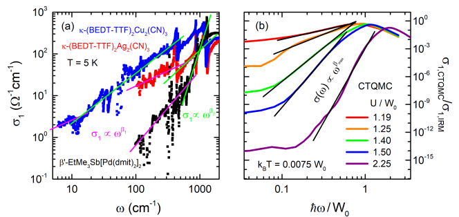
FIG. 1: (a) The in-gap conductivity of \beta' -EtMe 3 Sb-[Pd(dmit) 2 ] 2 , \kappa -(BEDT-TTF) 2 Ag 2 (CN) 3 and \kappa -(BEDT-TTF) 2 Cu 2 (CN) 3 can be approximated by power laws, as indicated by the straight lines in the double-logarithmic plot. Two different exponents are identified in different frequency regions. (b) Optical conductivity calculated by dynamical mean-field theory methods employing the continuous time quantum Monte Carlo (CTQMC) quantum impurity solver for different correlation strength U/W as indicated. The assumed k_B T/W = 0.0075 corresponds to the low-temperature limit of our experiments. \sigma_1(\omega) is normalized to the Ioffe-Regel-Mott limit \sigma_{\text{IRM}} and levels off towards the dc conductivity at low frequencies. Consistently, the exponents increase and \sigma_{dc} decreases with correlation strength.
