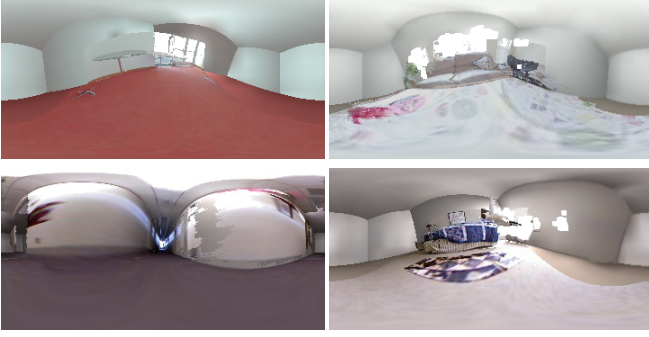
Fig. 8. Recovered environment maps of four test scenes.
