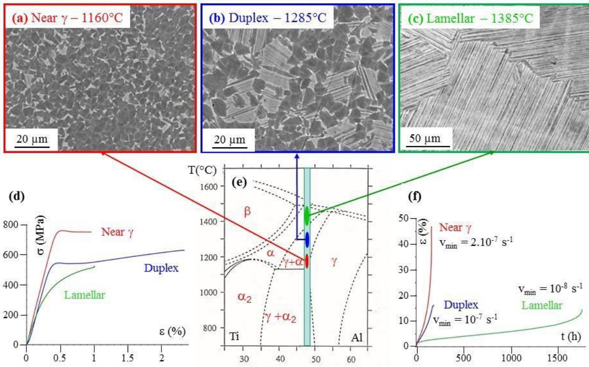
Fig. 2. Microstructures (a-c) and mechanical properties (d,f) of various GE48-SPS samples obtained at different temperatures as marked on the binary phase diagram (e).
