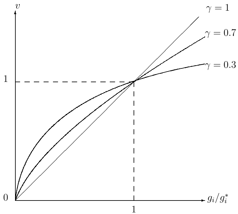
Figure 1: Behavior of v(g_i/g_i^*) = (g_i/g_i^*)^\gamma with different values of \gamma ( 0 < \gamma < 1 ).
