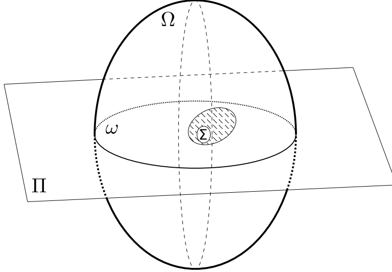
Figure 1: Buried planar crack
