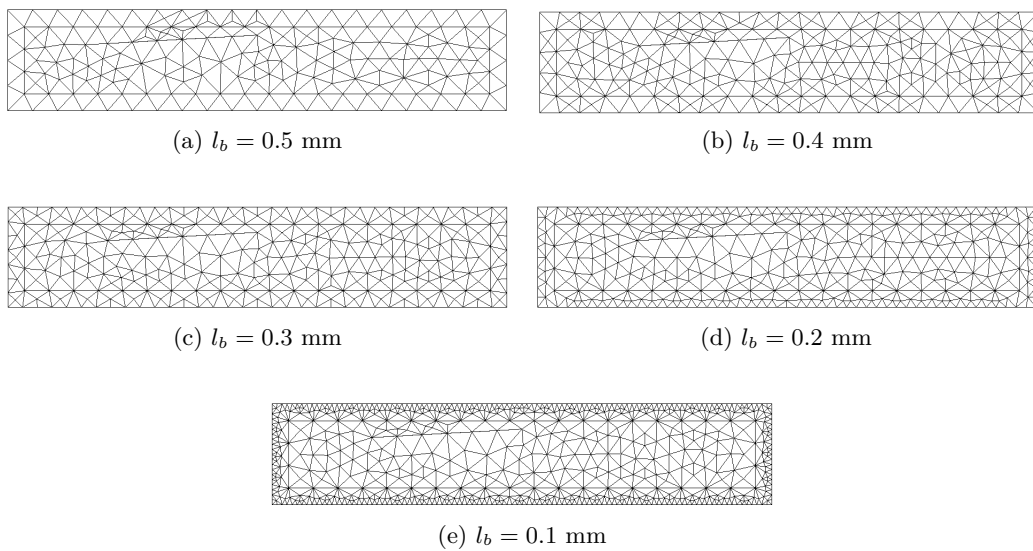
Figure 9: Different meshes used for the refinement study
