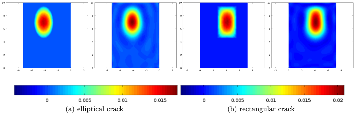
Figure 15: Identification of different shapes. h = 2 mm
