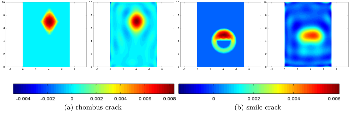
Figure 16: Identification of different shapes. h = 2 mm
