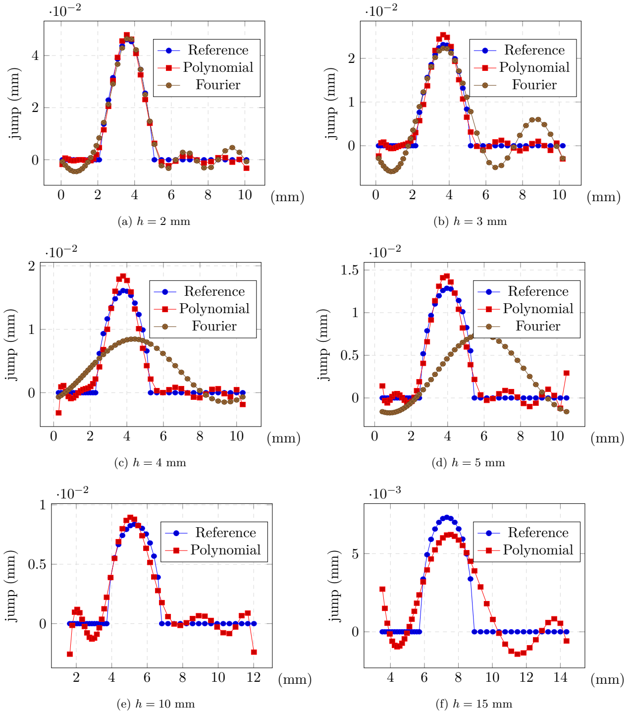
Figure 7: Identification of [[u_r]] \cdot n_{II} in \omega for various thicknesses in the absence of noise
