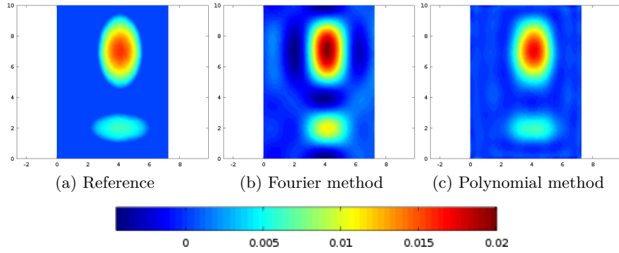
Figure 11: Reference and reconstruction of the gap for h = 2 mm
