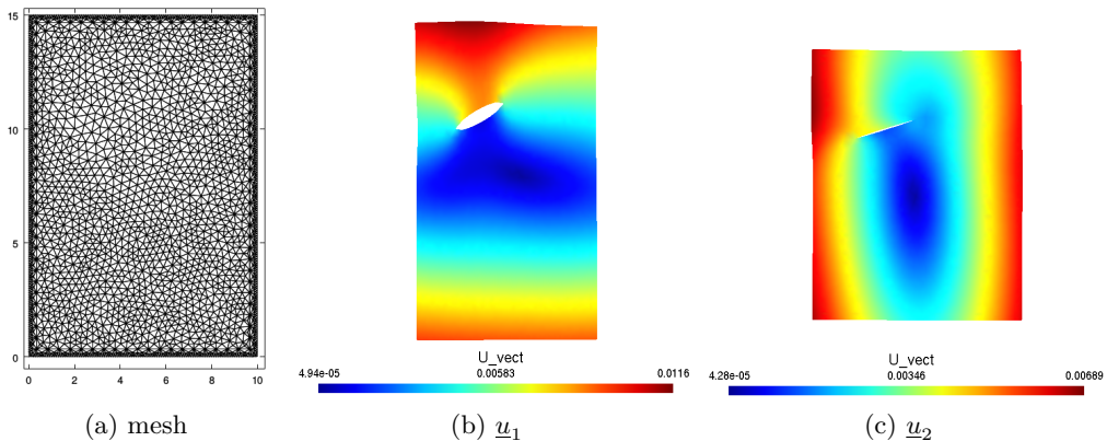
Figure 2: Example of FE mesh for the direct resolution, and solution (amplification \times 100 )
