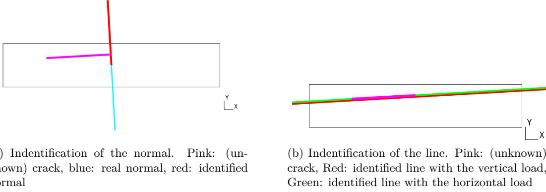
Figure 3: Thin 2D domain ( h = 2 mm) in the absence of noise, identification of the line.
