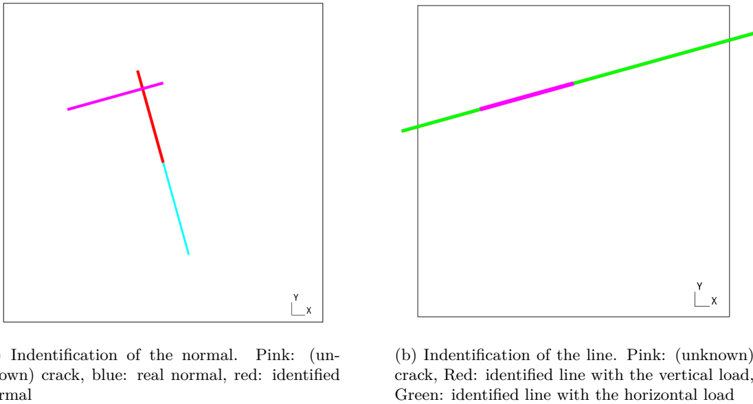
Figure 4: Thick 2D domain ( h = 10 mm) in the absence of noise, identification of the line.
