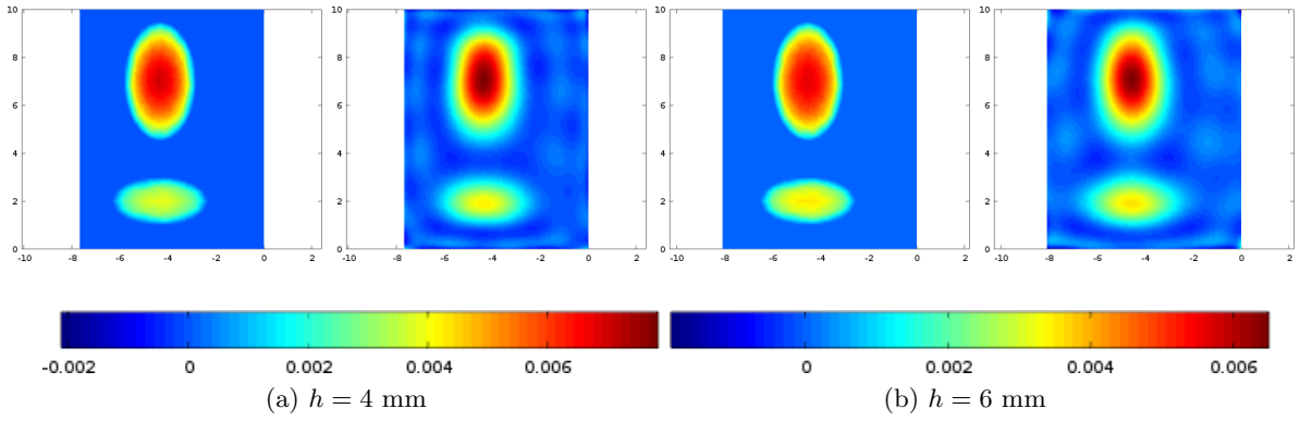
Figure 13: Reference compared to the polynomial identification
