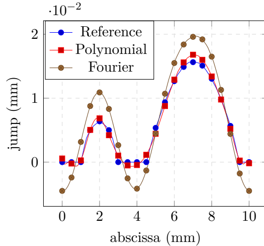
Figure 12: Reference and reconstruction of the gap on the line x = 4 mm with h = 2 mm
