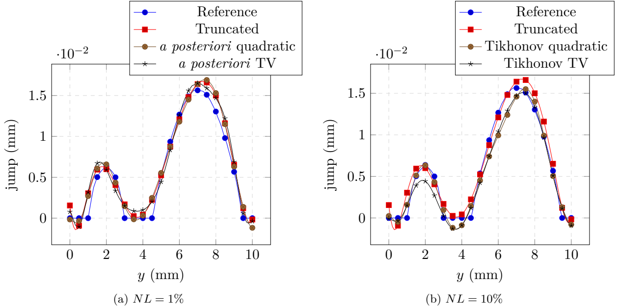
Figure 18: Reference and solution with different regularization techniques ( h = 2 mm) on the line x = -4 mm
