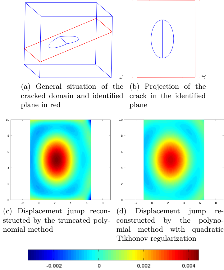
Figure 19: Identification of a non-planar crack in a 6 mm thick domain
