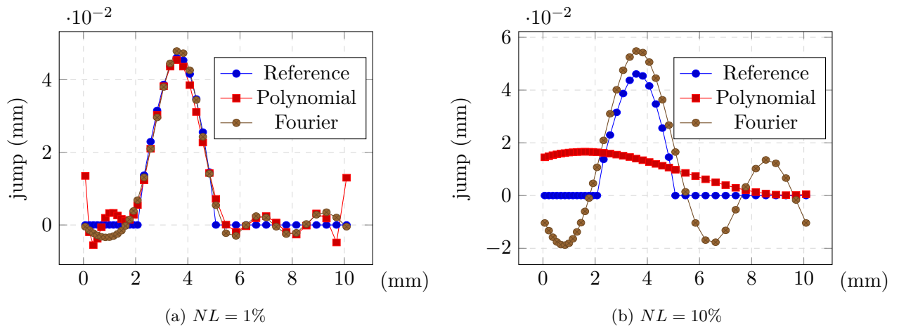
Figure 8: Identification of \llbracket u_r \rrbracket \cdot \underline{n}_{II} in \omega for thicknesses h = 2 mm with noise
