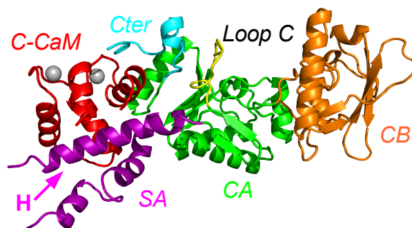
Figure 1. X-ray crystallographic structure (1YRT: [2]) of the complex AC/C-CaM. The AC domain includes three main subdomains, named CA (green), CB (orange), and switch A (SA) (purple). The switch A is named according to the three switches A, B and C, displaying large conformational changes [1] during the Edema Factor (EF) conformational transition. In AC, the regions corresponding to the EF switches were marked by Guo and coworkers [2]. The region corresponding to the switch C is the C terminal tail (cyan), and the one corresponding to the switch B is the catalytic loop (yellow). The two regions are included in the domain CA. The residue definitions of the regions are the following: residues 1–55, 181–191, 255–293 and 307–339 for CA excluding the C-terminal tail and the catalytic loop, residues 294–306 for the catalytic loop, residues 340–358 for the C terminal tail, residues 56–180 for CB, residues 192–254 for SA. These numbers are reduced by 6 for the residue numbers in 1YRT.
