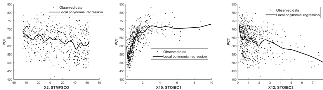
Fig. 4. Scatterplots with local polynomial regression of PCT according to several inputs, from the learning sample of n = 500 simulations.
