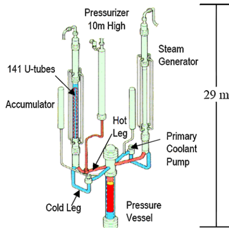
Fig. 1. Hot and cold legs of the Large Scale Test Facility.
