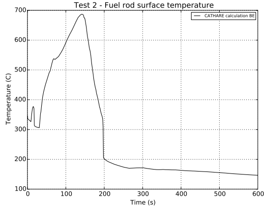
Fig. 2. Physical simulation output of the model with CATHARE code: maximal rod cladding temperature during the transient.
