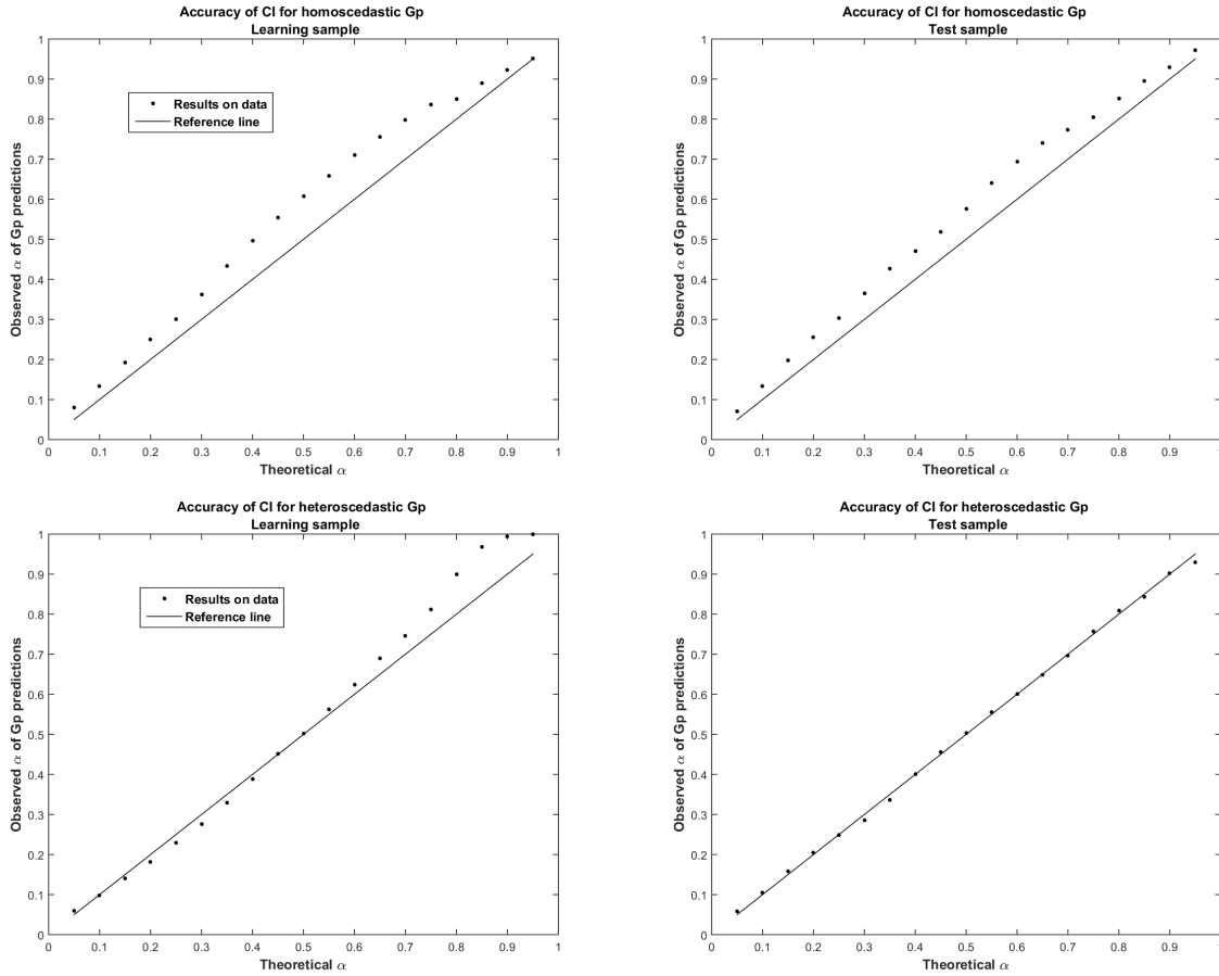
Fig. 5. Proportion of observations that lie within the \alpha -confidence interval predicted by the Gp, according to the theoretical \alpha . Top: results for homoscedastic Gp ( Gp_{m,1} ) on the learning sample (left) and on the test sample (right). Bottom: results for heteroscedastic Gp ( Gp_{m,2} ) on the learning sample (left) and on the test sample (right).
