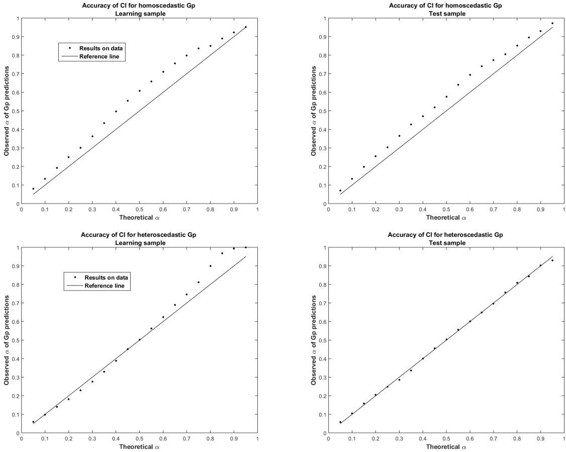
Fig. 5. Proportion of observations that lie within the \alpha -confidence interval predicted by the Gp, according to the theoretical \alpha . Top: results for homoscedastic Gp ( Gp_{m,1} ) on the learning sample (left) and on the test sample (right). Bottom: results for heteroscedastic Gp ( Gp_{m,2} ) on the learning sample (left) and on the test sample (right).
