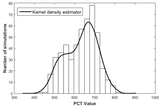
Fig. 3. Histogram of the PCT from the learning sample of n = 500 simulations.
