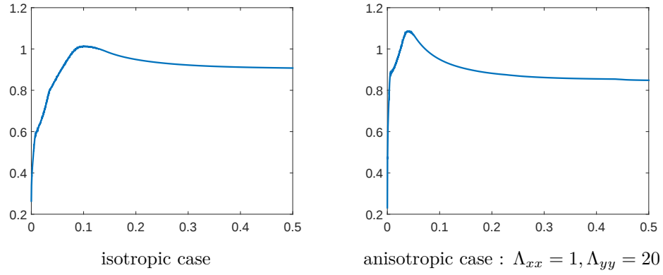
FIGURE 6. Control of the entropy.
