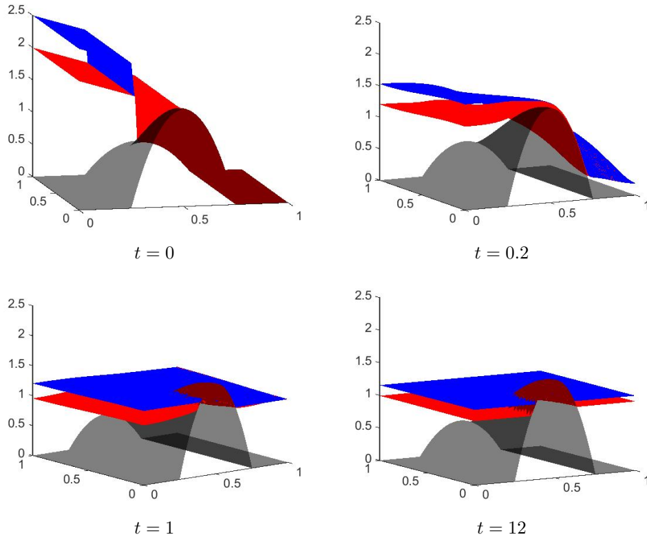
FIGURE 4. Behaviour of the model with an isotropic tensor \Lambda = \mathbf{I} .
