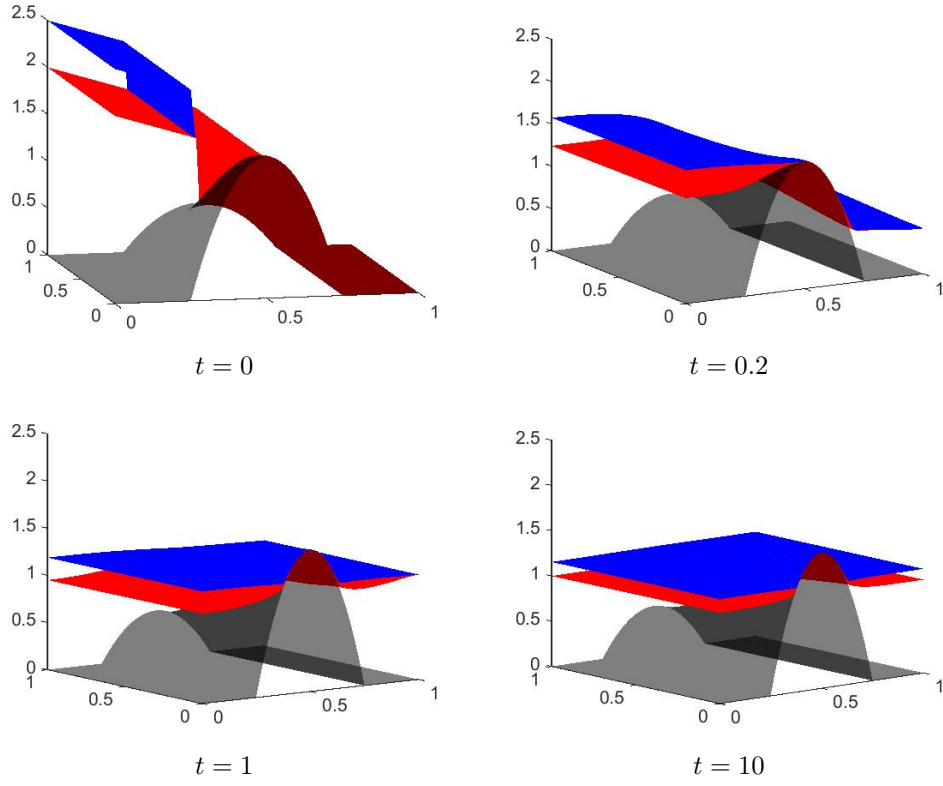
FIGURE 5. Behaviour of the model with an anisotropic tensor : \Lambda_{xx} = 1, \Lambda_{yy} = 20 .
