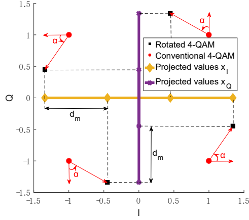
Fig. 2. Uniformly projected RCQD 4-QAM signal
