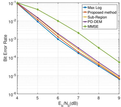
Fig. 6. BER performance of several algorithms for uniformly projected RCQD 4-QAM signal on KAU2
