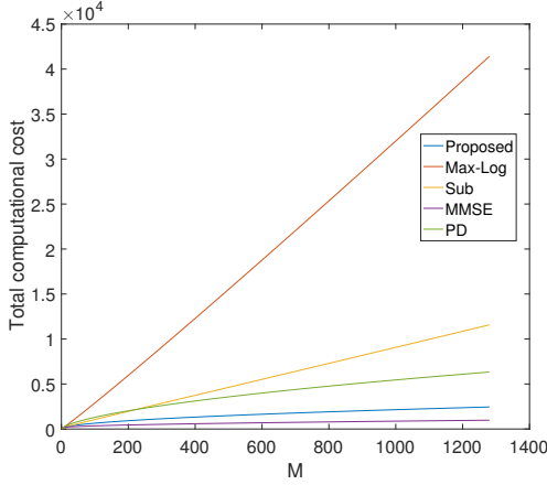
Fig. 4. Complexity comparison of several demappers
