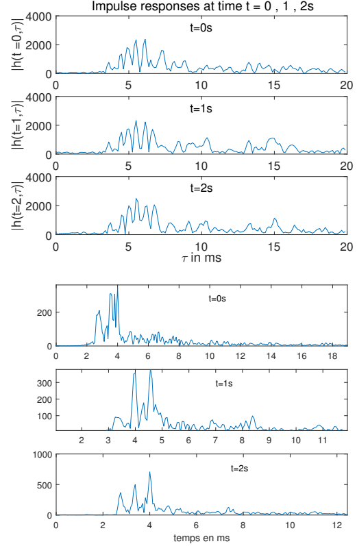
Fig. 3. Impulse responses at times t = 0, 1 and 2 s of KAU2(up) and NOF1(bottom)
