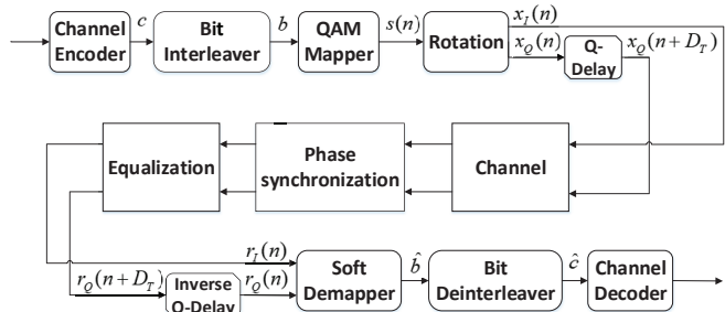
Fig. 1. Underwater acoustics system model with RCQD constellation
