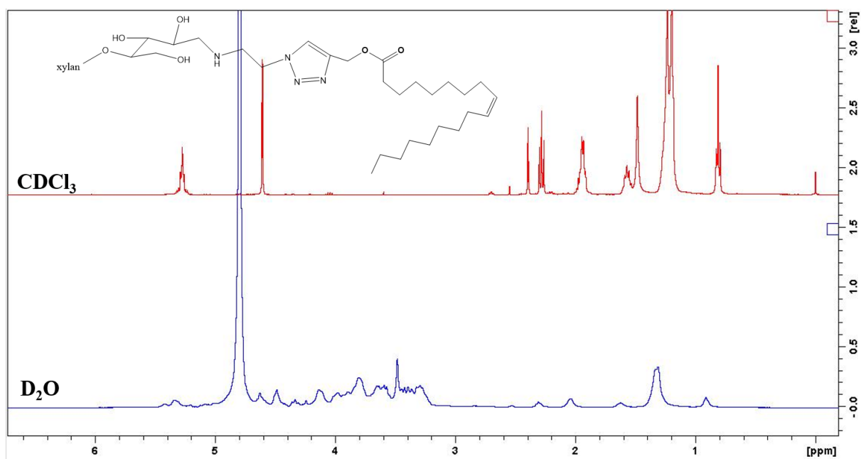
Supporting Figure S8. Overlaid spectra of the ^1\text{H} NMR of the bioconjugate XOS- b -MeOl in \text{CDCl}_3 (top) and in \text{D}_2\text{O} (bottom).
