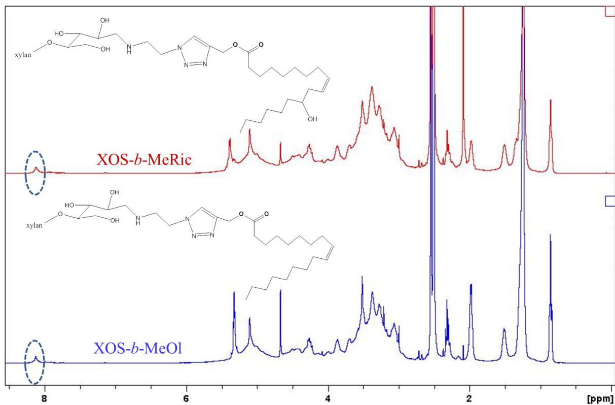
Fig. 3 Overlaid spectra of the ^1\text{H} NMR of the bioconjugates XOS- b -MeOl (bottom) and XOS- b -MeRic (top) in DMSO- d_6 .
