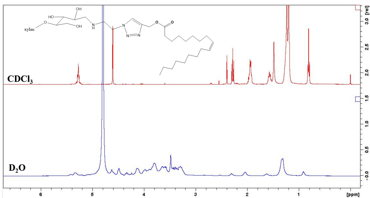
Supporting Figure S9. Overlaid spectra of the ^1\text{H} NMR of the bioconjugate XOS- b -MeRic in \text{CDCl}_3 (top) and in \text{D}_2\text{O} (bottom).
