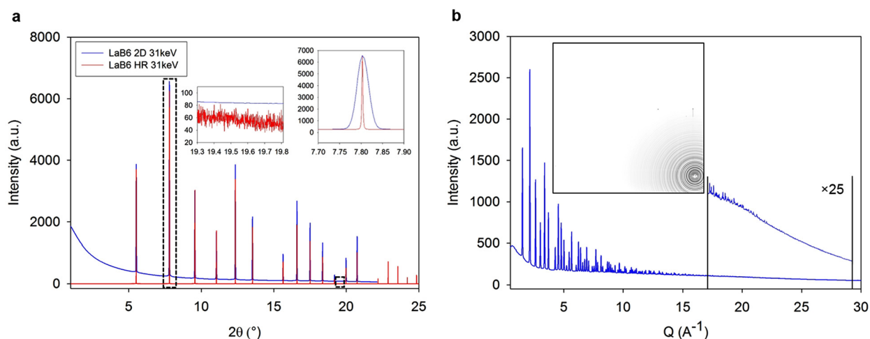
Fig. 2. a) Comparison between two powder diffraction patterns of \text{LaB}_6 (NIST, 660b) measured with the high-resolution setup (HR) and a flat panel PerkinElmer XRD 1611 detector (2D, 41 \times 41 \text{ cm}^2 ) at an energy of 31 keV. The intensity has been normalized using the 110 reflection (most intense peak, see inset). b) Powder diffraction pattern of \text{LaB}_6 measured for PDF analysis at an energy of 70 keV using the flat panel PerkinElmer detector. By integrating the 2D pattern along the diagonal, a Q_{\text{max}} of 29 \text{ \AA}^{-1} is accessible.
