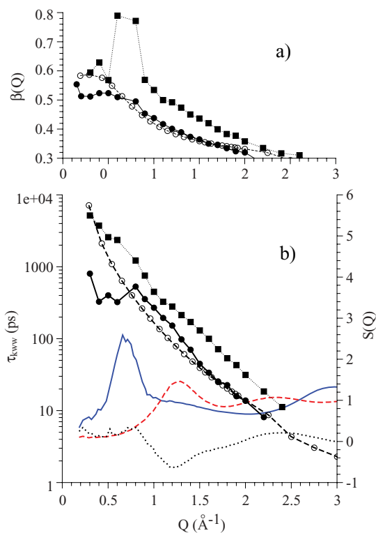
FIG. 14. Q dependence of the parameters of the KWW fitting the coherent intermediate scattering functions in the coarse-grained analysis at 650 K: (a) stretching parameter (b) KWW characteristic time. Full squares represent the MC subsystem, full circles the SG subsystem. The results for the self-correlation function of SG center of mass are also shown as empty circles for comparison. In (b), lines show S_{\text{MC/MC}}^{\text{CoM}}(Q) (solid blue), S_{\text{SG/SG}}^{\text{CoM}}(Q) (dashed red), and S_{\text{MC/SG}}^{\text{CoM}}(Q) (dotted black).
