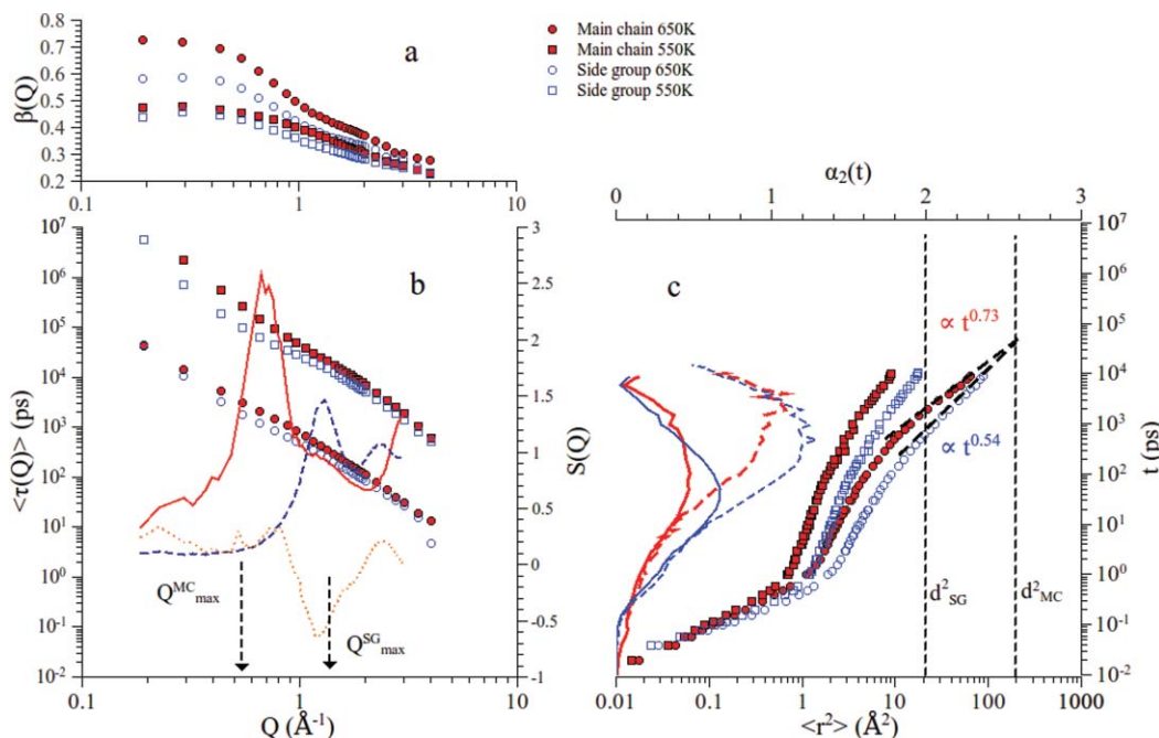
FIG. 12. Results of the coarse-grained analysis at 550 and 650 K. Fits of Eq. (11) to F_{MC}^s(Q, t) and F_{SG}^s(Q, t) deliver the stretching parameters and average relaxation times shown as symbols as function of Q in (a) and (b), respectively. In (b), the vertical arrows indicate the cross over between dynamical regimes, and the lines show the structure factors at 650 K (solid: MC/MC correlations; dashed: SG/SG correlations; dotted: MC/SG correlations). (c) Mean squared displacement (Filled symbols: MC; Empty symbols: SG) for the two subgroups. The non-Gaussian parameters are also shown as lines (solid for 550 K and dashed for 650 K; thin for SG and thick for MC). The time scale on the ordinate axis is the same as in (b). The dashed vertical lines mark the values corresponding to d_{SG}^2 = 23 \text{ \AA}^2 and d_{MC}^2 = 110 \text{ \AA}^2 .
