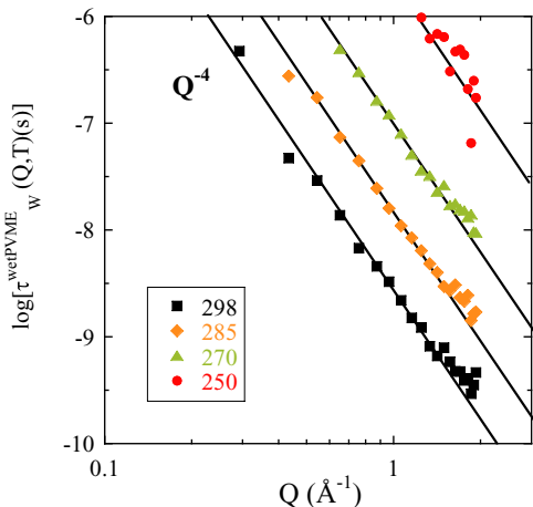
FIG. 7. Momentum transfer dependence of the characteristic times of the PVME component in the solution obtained by fixing \beta^{PVME} = 0.3 . Solid lines show a Q^{-4} -dependence.
