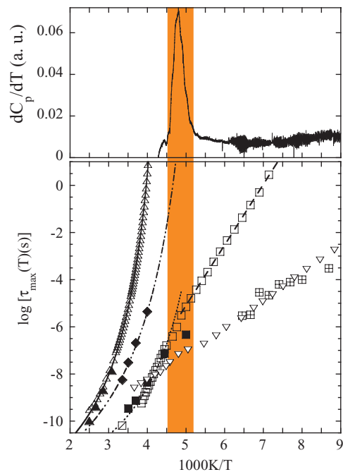
FIG. 3. (a) Derivative of the specific heat of PVME/H 2 O as function of the inverse temperature. (b) Relaxation map of the PVME/H 2 O system. Filled symbols: NS characteristic times at Q = 1\text{\AA}^{-1} for the PVME ( \blacklozenge ) and water ( \blacksquare ) components. Empty symbols: DS relaxation times for the slow ( \square ) and fast ( \circ ) processes. Results obtained on dry PVME are shown for comparison: \alpha - ( \triangle ) and \beta -process ( \nabla ) observed by DS, and NS characteristic times at Q = 1\text{\AA}^{-1} ( \blacktriangle ) (Ref. 27). The time corresponding to the maximum of the associated distribution has always been represented to compare results corresponding to different spectral shapes. Solid, dashed-dotted, and dotted lines are VF laws (see text) and the dashed line is an Arrhenius fit to the “slow” process below 200\text{ K} . Shaded area indicates the region of the calorimetric glass-transition in the wet PVME system.
