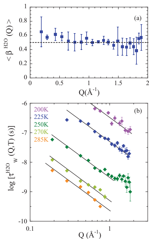
FIG. 8. Momentum transfer dependence of the T -averaged shape parameter (a) and the characteristic times (b) of the water component in the solution obtained by fixing \beta^{PVME} = 0.3 . Dotted line in (a) marks the value \beta = 0.5 and solid lines in (b) show Q^{-2} -dependencies.
