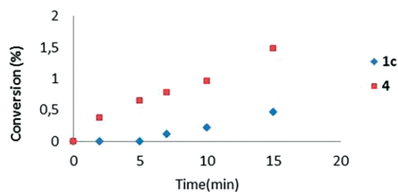
Figure 3. Compared kinetic profiles of the reaction at room temperature using 1c or 4 in early times of the reaction – conversions were measured by ^1\text{H} NMR spectroscopy. Profiles obtained by the arithmetic mean of 3 experiments.
