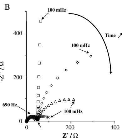
Fig. 4. Evolution of the Nyquist plots with the polarization time; A. titanium rod electrode, B. "titanium rod-carbon felt" system, both inoculated with salt marsh sediment and under polarization at 0.1 V/SCE.
