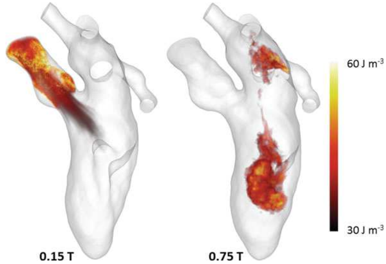
Fig. 9 3D volume rendering of the FKE in the left heart during systole ( left , 0.15 T) and diastasis ( right , 0.75 T). The opacity is set to 0% for FKE values below 30 \text{ J m}^{-3} . The mitral and aortic valves are not displayed for more clarity but were accounted for in the simulation
