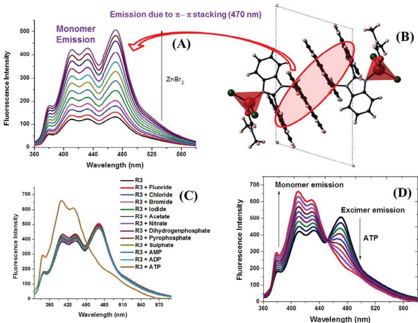
Figure 4: (A) Change in emission profile of ligand L3 (10 μM) upon addition of 15 μM of Zinc bromide in DMF: water (30:70) HEPES buffer (B) Packing of complex 3 , showing π-π stacking interaction between pyrene rings. (C) Change in emission profile of complex 3 (10 μM) upon addition of 16 μM of various anions in HEPES buffer (DMF: water) (d) Change in emission profile of complex R3 with successive addition of ATP (0-16 μM).
