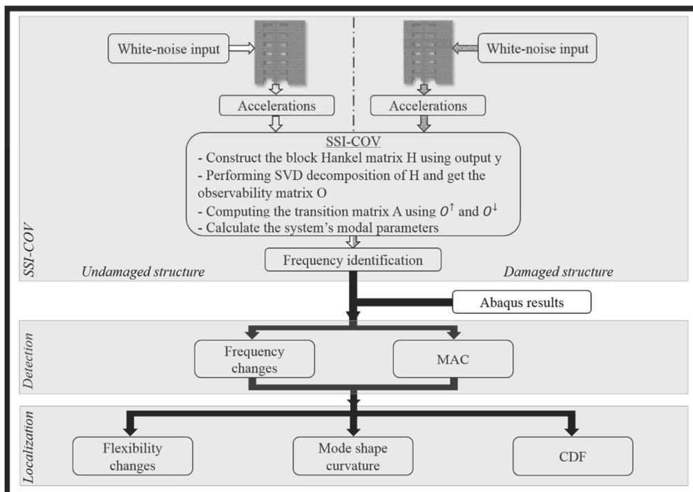
Fig. 4 - Flowchart of numerical simulation
