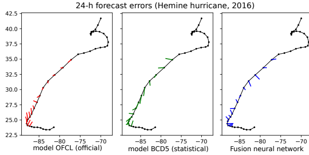
Figure 4: 24-h forecast errors (4 time steps ahead) on Hermine hurricane in 2016. The bars connect each pair of predicted and ground truth location. The larger the length, the larger the error.
