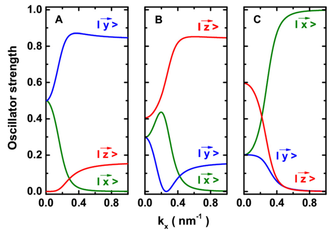
FIG. 5. Triptych representation of the expansion of A (left), B (middle), and C (right) levels against k_x . At high values of k_x , the ground state valence band (A) is dominantly built from |y\rangle Bloch state and from about 15 percents |z\rangle state. The second level (B) is dominantly built from |z\rangle Bloch state and from about 15 percents |y\rangle state. Note the quasi similar expansion of A and B through |y\rangle and |z\rangle , respectively. Last for high values of k_x , it appears the C is built of |x\rangle Bloch state only. These expansions impact the selection rules for band to band transitions.
