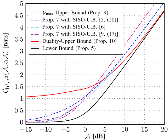
Fig. 1. Bounds on the capacity of the MISO channel with three LEDs and channel gains \mathbf{h} = (3, 2, 1.5) for the case \alpha = 0.6 . Note that the threshold of this channel is \alpha_{\text{th}} = 1.2692 (and \frac{n_T}{2} = 1.5 ). The upper bound from Proposition 7 is plotted in combination with three known SISO capacity bounds taken from [5], [6], and [9]. Note that the bound from [9] is only valid for \mathcal{A} \leq -1.97 dB.
