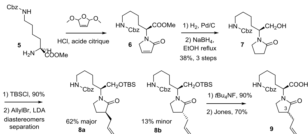
Scheme 1: synthesis of the key product 9
