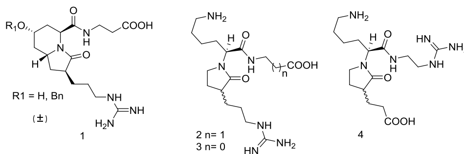
Figure 1: RGD peptidomimetics
