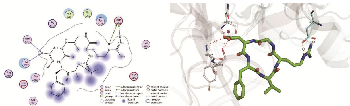
Figure 2 : LigX 2D-depiction (left side) and 3D-representation focused on Arg and Asp side chains (right side) of the binding mode of cyclo(RGDF=N{Me}V) to integrin alpha V beta 3 in PDB 1L5G
