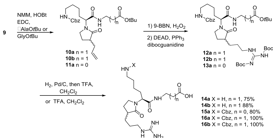
Scheme 2: introduction of acid and basic moiety
