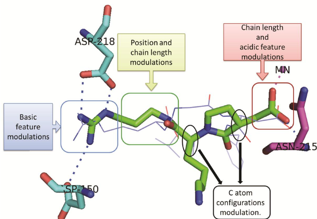
Figure 3 : Structural basis of in silico optimization of peptidomimetics
