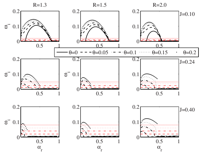
FIG. 13. (Color online) Amplification rates \omega_j vs the wavenumber for fixed values of the Richardson number J and for different values of the density scale parameter R . The larger amplification rates are those of \mathcal{KH} instabilities.
