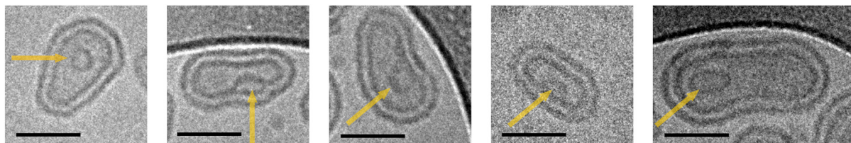
Figure S3. Cryo-TEM images of PDMS-g-PEO nested vesicles with the internal buds (showed by arrows) resulting from the membrane fusion and budding. Scale bars represent 50 nm.
