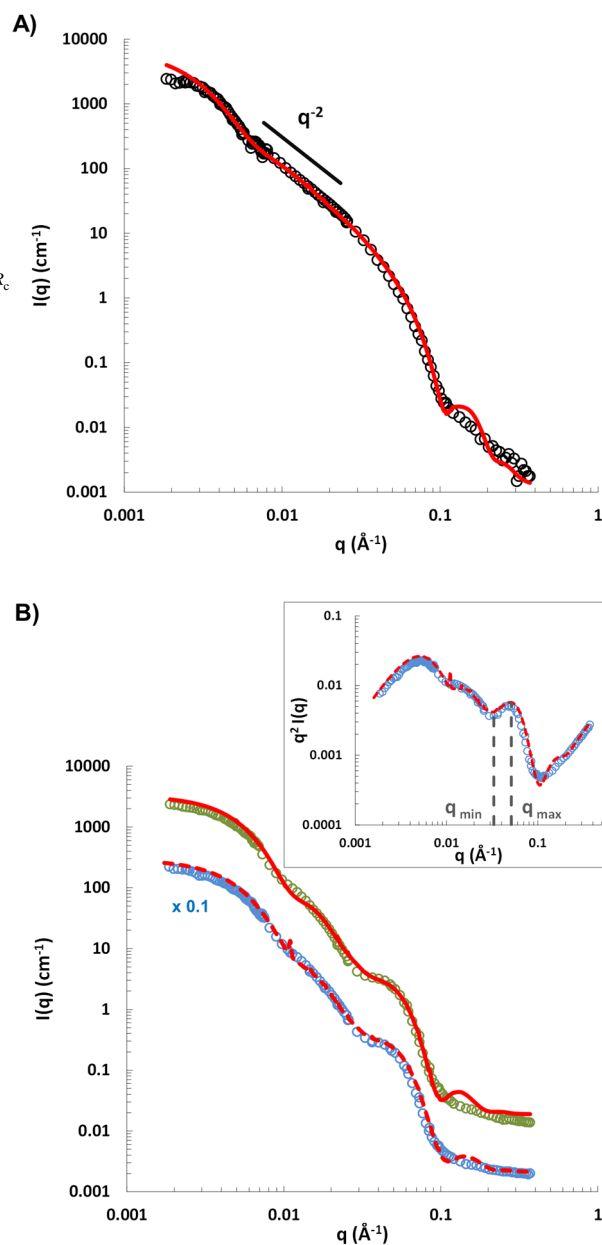
Figure 3. Small angle neutron scattering of PDMS-g-PEO vesicles initially prepared at 10 mg/mL in D_2O . A) Experimental data in isotonic conditions, the full line is a fitting curve by a polydisperse hollow spheres
