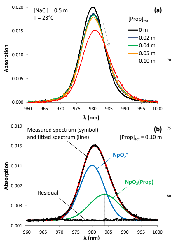
Fig. 1(a) Np(V) absorption spectra for various propionate concentrations (0–0.3M) at [\text{Np(V)}]_{\text{tot}} = 5.94 \times 10^{-5} M, I = 0.51 m; T = 23^\circ\text{C} . b) Example of a deconvoluted spectrum ( [\text{Prop}] = 0.1 m; I = 0.51 m; pHc = 5.0, T = 23^\circ\text{C} ).
