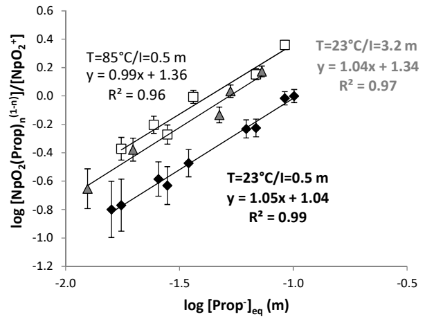
Fig. 2 Slope analysis of the Np(V)-propionate complex formed at 23 and 85°C for [\text{NaCl}] = 0.51 \text{ m} , and 23°C for [\text{NaCl}] = 3.2 \text{ m} . Slopes \approx 1 ( 1.05 \pm 0.05 and 0.99 \pm 0.11 for both T, respectively, 1.04 \pm 0.15 for I = 3.2 m) indicate the formation of the 1:1 complex. Log \beta (conditional) increases both with temperature and ionic strength (from 1.04 \pm 0.06 to 1.36 \pm 0.13 ).
