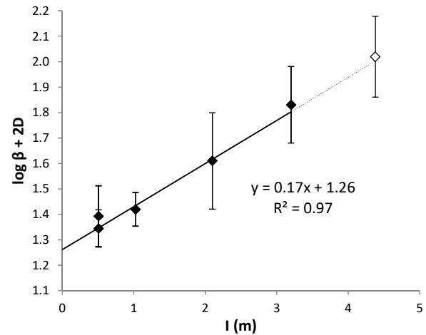
Fig. 3 SIT plot of the equilibrium reaction \text{NpO}_2^+ + \text{Prop}^- \rightleftharpoons \text{NpO}_2(\text{Prop}) in NaCl, yielding \log \beta_0 = 1.23 \pm 0.03 . The white symbol ( [\text{NaCl}] = 4.2 \text{ m} ) shows data outside the recommended applicability of the SIT (data not used in the regression). The dotted line shows the extrapolation of the results obtained for lower I to 4.2 m.
