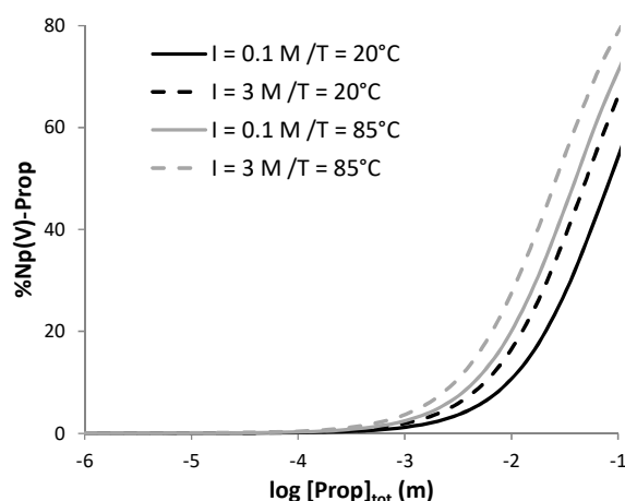
Fig. 6 Calculated percentage of Np(V)-propionate complex ( [\text{Np(V)}]_{\text{tot}} = 10^{-10} \text{ m} ) versus \log [\text{Prop}]_{\text{tot}} for \text{pH}_c = 7 and I = 0.1 or 3 m and T = 20 or 85^\circ\text{C} using thermodynamic parameters determined in this study.
