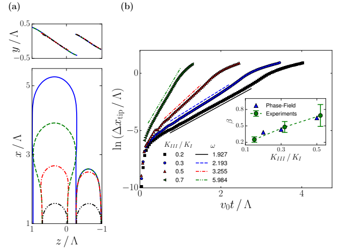
FIG. 4: (Color online). (a) Illustration of spatial period doubling instability in a phase-field simulation for K_{III}/K_I = 0.5 ; out-of-plane and in-plane projections of crack fronts at different times are plotted in the top panel and the bottom panel, respectively (see Movie 3 of [29]). (b) Semi-log plot of difference of tip positions along the propagation x -axis between leading and lagging facets versus scaled time for different K_{III}/K_I . Inset: coarsening rate \beta versus K_{III}/K_I obtained from experiments and phase-field simulations. In all simulations, D_x = 307\xi , D_y = 60\xi , D_z = 120\xi , \Lambda = 60\xi and G = 1.5G_c .
