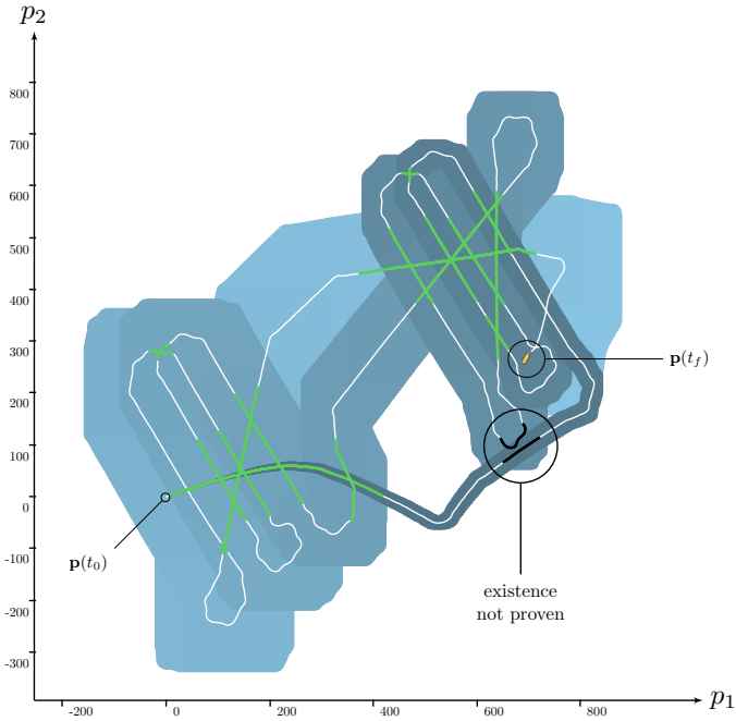
Figure 13: 2D trace of Redermor AUV. The projected tube [p](\cdot) (i.e. the bounded estimated positions) is drawn in blue, depicting an increasing localization uncertainty. The truth is plotted by the white line while green and black lines are the projections of the results given by the topological degree test \mathcal{T} .
