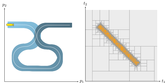
Figure 7: Guaranteed loop detections of a mobile robot. Several evolutions are drawn on the left hand side: the true trajectory is plotted in white while the computed envelope of all feasible trajectories is represented in blue, depicting some localization uncertainties due to measurement errors. Parts of the corresponding t -planes are pictured on the right hand side with the loop detection set \mathbb{T} approximated by a set of boxes [t]_j . This reliable approximation is obtained with a SIVIA algorithm. When an actual loop \mathbf{t}^* exists – pictured by a black dot – it is surely enclosed by this set of boxes.
