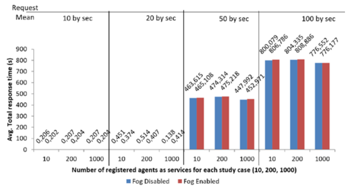
Fig.6. Average total response time vs number of registered agents as services.
