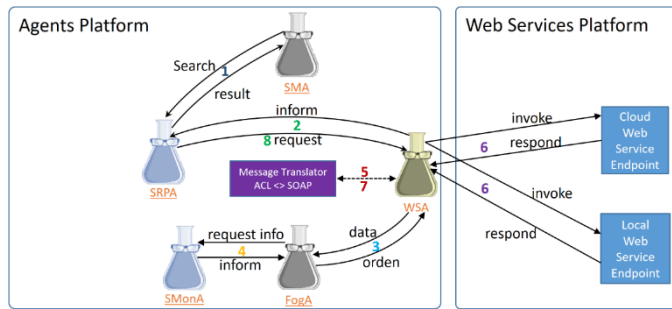
Fig 3. Fog interaction between agents.
