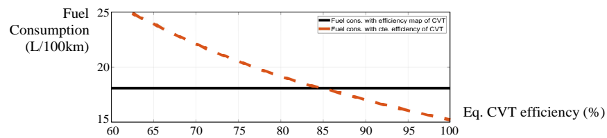
Fig. 5. Comparison of equivalent constant efficiency with a variable efficiency of the CVT
