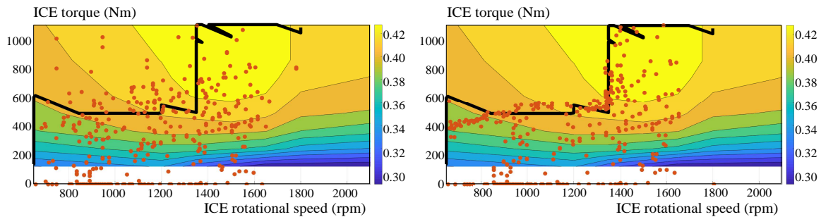
Fig. 7. ICE operation points of the studied HETs on the ICE efficiency map: a) AMT-based HET, b) CVT-based HET
