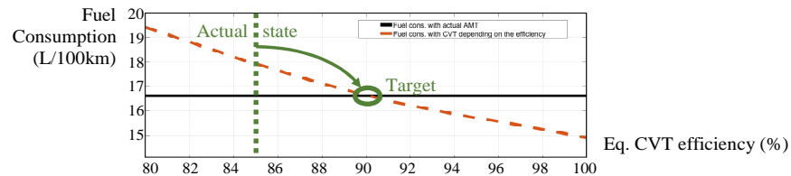
Fig. 9. Influence of the equivalent constant CVT efficiency on the fuel consumption
