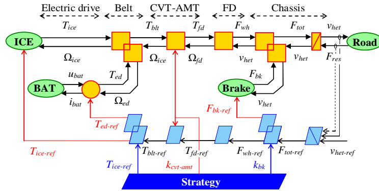
Fig. 3. Common EMR of the studied AMT-based or CVT-based HETs
