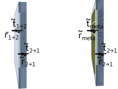
FIG. 2 Schematic showing the Fresnel coefficients for the simple layer (left), and the metasurface (right) as in equation (9).
