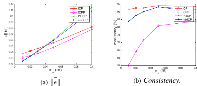
Fig. 9: Mean of the norm of the relative position error \|\bar{\epsilon}\| and consistency for the four matchings depending on the LiDAR range noise with a standard deviation \sigma_\rho .
