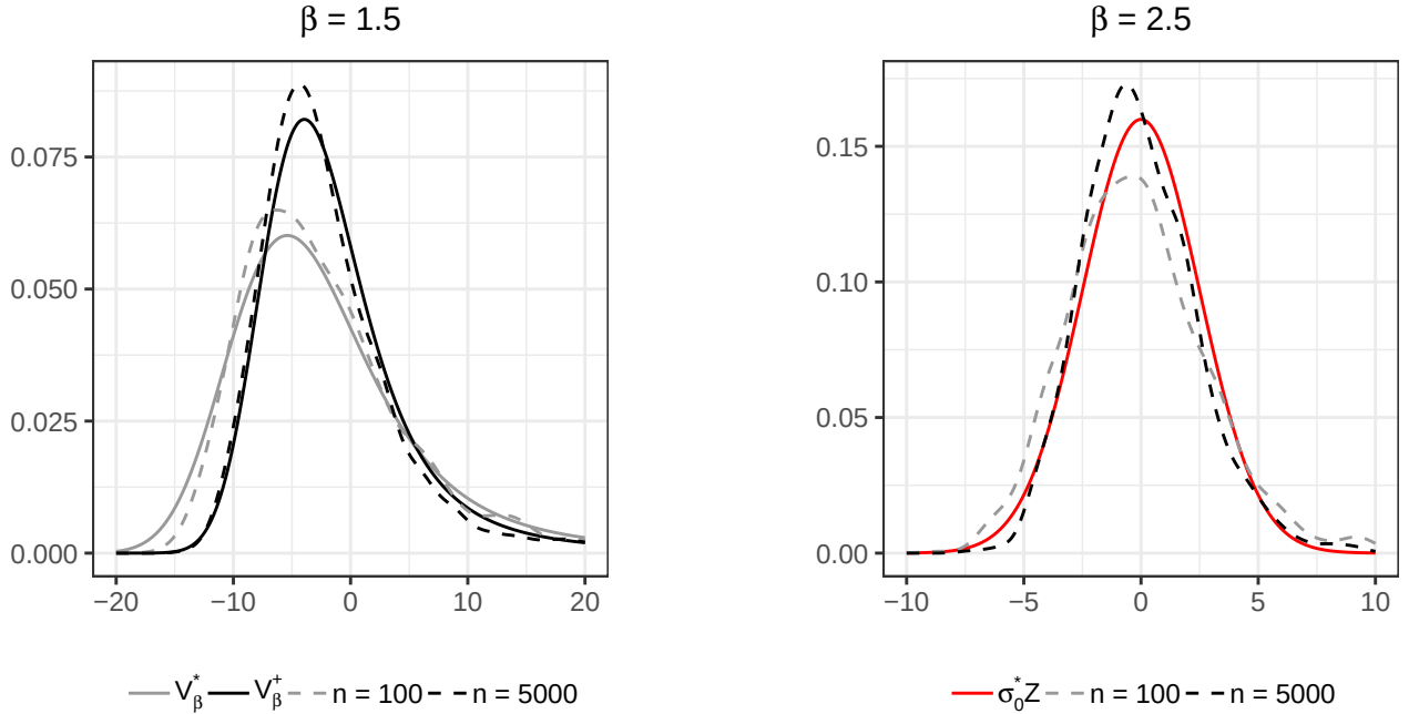
Figure 1: Density of the limiting random variables in cases [left] (i),(ii), [right] (iv) of Corollary 4.1 for t = 0 and their kernel density estimates constructed from a random sample of size 1000 from \hat{\gamma}_{N,n}(0, 0) in (1.6) with N = 5000 , a^2 \sim \text{Beta}(2, \beta) , \varepsilon(0) \sim N(0, 1) .
