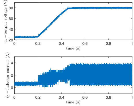
Figure 15. Output voltage (a) and inductor current (b) during a start-up test by means of PI control strategy.
