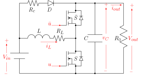
Figure 1. Synchronous boost converter.
