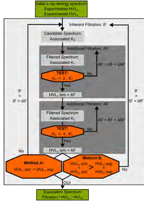
Fig. 2. Flowchart for the experimental determination of the CT model.
