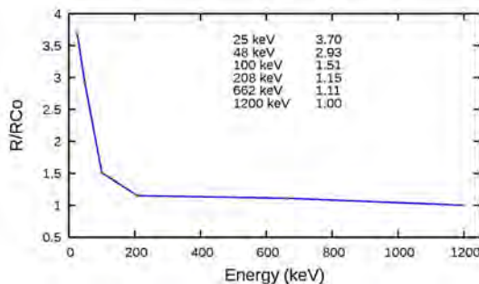
Fig. 9. Energy dependence of OSL detectors.
