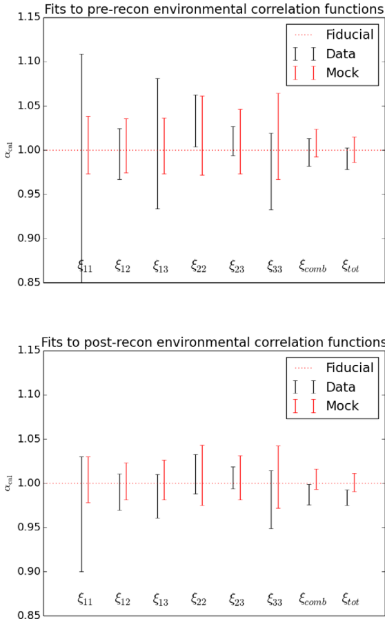
Figure 5. The 68 per cent confidence range of the fits of \alpha_{\text{cal}} to the pre-reconstruction (upper panel) and post-reconstruction (lower panel) autocorrelation and cross-correlation function measurements \xi_{IJ} of the CMASS DR12 galaxy data set, in three environmental slices defined by increasing local density. The mean and standard deviation of the best-fitting values of \alpha_{\text{cal}} for the ensemble of QPM mock catalogues are also displayed. The last two pairs of results show the results of fitting a single \alpha_{\text{cal}} value to the set of measurements in different environments, including the appropriate covariance ( \xi_{\text{comb}} ), and to the total galaxy correlation function ( \xi_{\text{tot}} ). These procedures produce similar final results. The QPM mock mean template is used to construct the BAO model, although the results are not sensitive to this choice.
