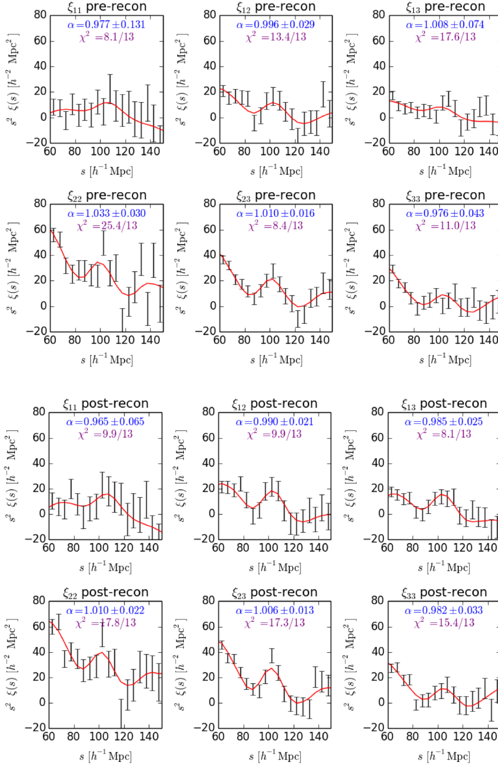
Figure 3. Autocorrelation and cross-correlation function measurements \xi_{IJ} of the CMASS DR12 galaxy data set in three environmental slices defined by increasing local density. The upper and lower sets of panels display results before and after reconstruction, respectively. The solid line is the best-fitting model in each case, using a template built from the corresponding QPM mock mean correlation function. We also show the 68 per cent confidence range of the posterior probability distribution of \alpha , and the \chi^2 statistic of the best-fitting model and number of degrees of freedom. Baryon acoustic peaks are detected in all six of the post-reconstruction environmental correlation functions.
