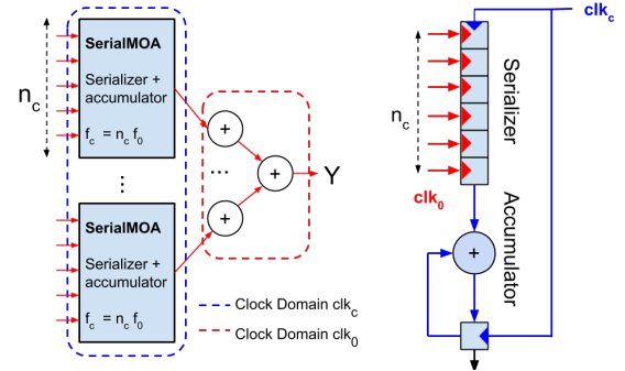
Figure 2: Architecture of a serial MOA. Each Serializer Accumulator Pair replaces a cluster of adders in the MOA of Figure 1
