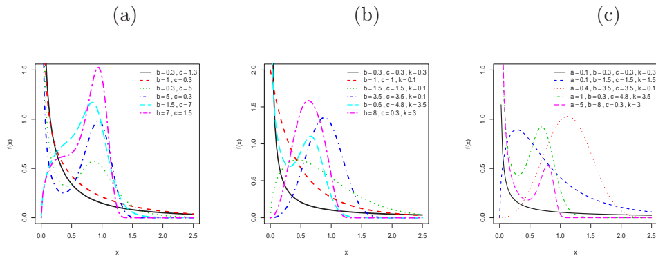
Figure 2: Plots of the minWB density for some parameter values.
