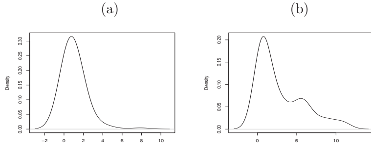
Figure 8: Gaussian kernel density estimation for data sets (a) Data set 3 (b) Data set 4.
