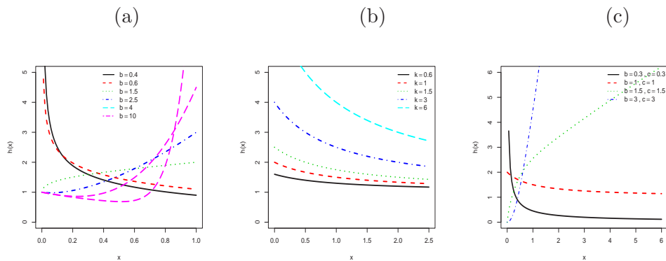
Figure 3: Plots of the minWB hazard rate for some parameter values.
