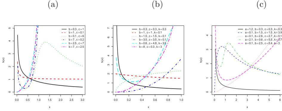
Figure 4: Plots of the minWB hazard rate for some parameter values.
