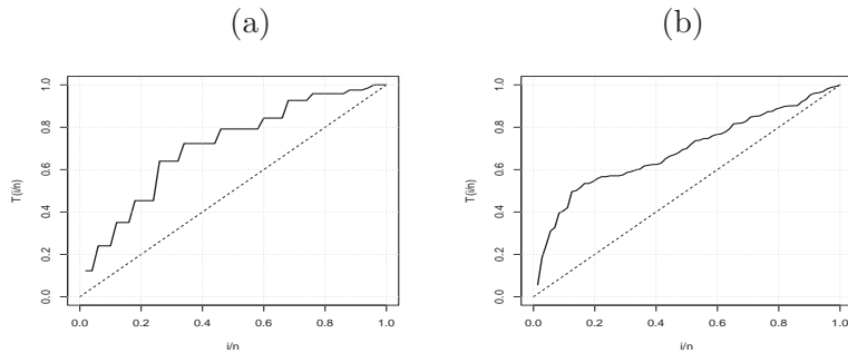
Figure 5: TTT plots for (a) Data set 1 (b) Data set 2.
