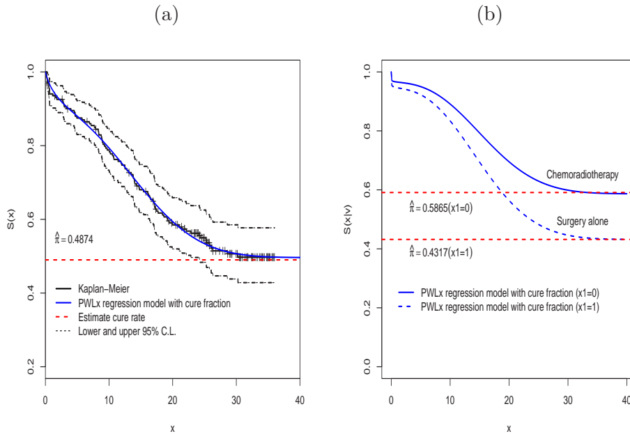
Figure 13: (a) Kaplan-Meier curves (solid lines), the estimated PWLx survival function and the estimated cure fraction for the gastric cancer data. (b) Estimates of the survival function and cure fraction of model stratified by type of therapy for the gastric cancer data.
