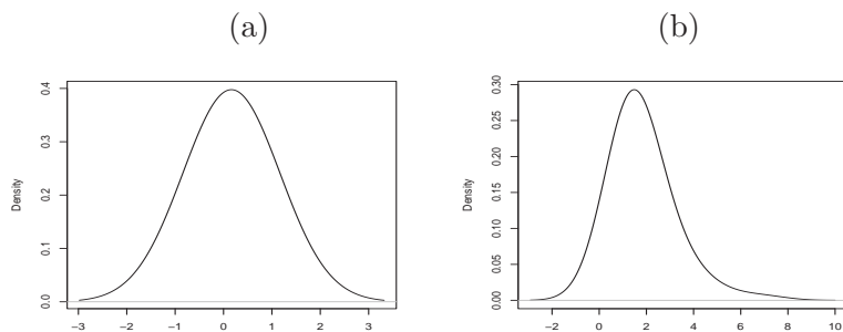
Figure 7: Gaussian kernel density estimation for data sets. (a) Data set 1 (b) Data set 2.
