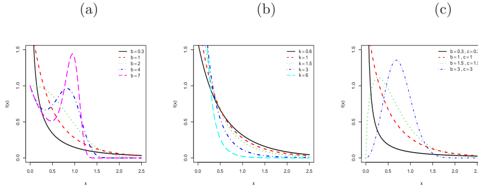
Figure 1: Plots of the minWB density for some parameter values.
