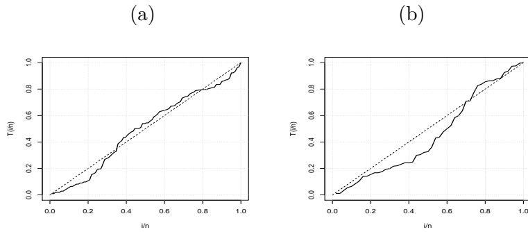
Figure 6: TTT plots for (a) Data set 3 (b) Data set 4.
